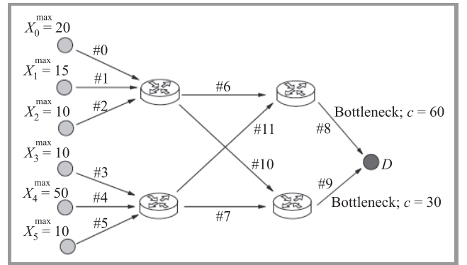
Fig. 1. Test network.
