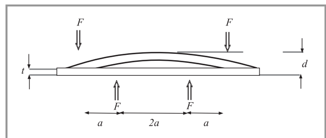
Fig. 1. Four-point bending setup.
