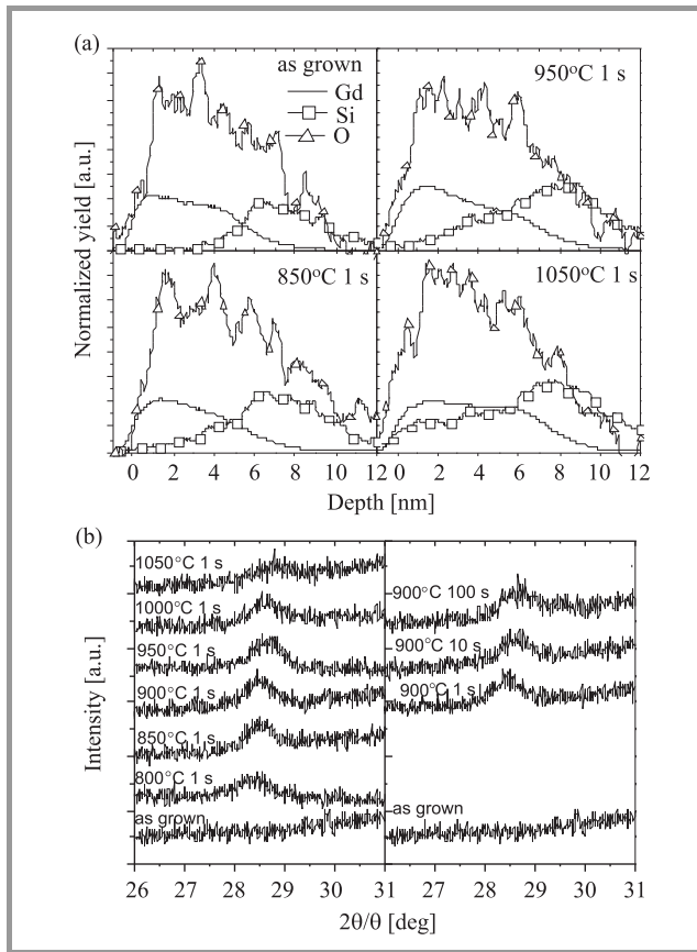
Fig. 4. (a) MEIS and (b) XRD profiles for ALD grown \text{Gd}_2\text{O}_3/\text{SiO}_2 gate stacks under different RTA conditions [65].
