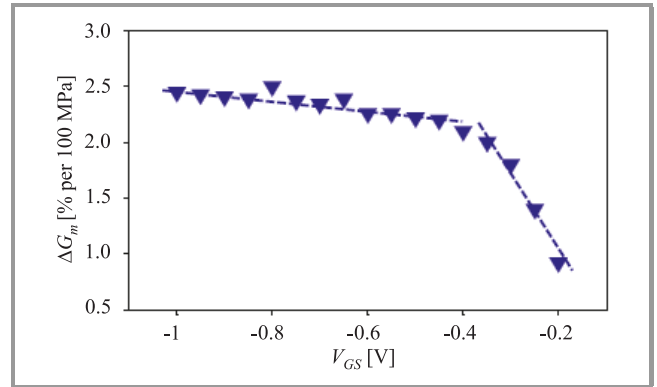
Fig. 8. Variation of dc transconductance G_m with the applied stress for PMOSFETs as a function of V_{GS} at V_{DS} = -1.2 V.
