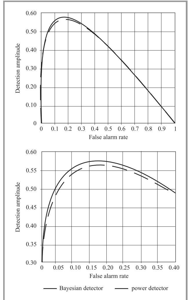
Fig. 2. Detection amplitude comparison in MIMO; M = 2 , N = 8 , L = 10 , \text{SNR} = -10 dB.
