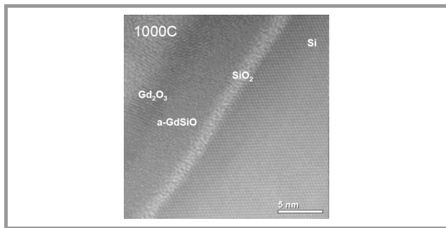
Fig. 5. HRTEM image of ALD bi-layer structure \text{Gd}_2\text{O}_3/\text{GdSiO}/\text{SiO}_2 after RTA at 1000^\circ\text{C} for 1 s in \text{N}_2 .
