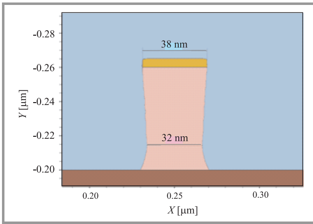
Fig. 3. Fin sidewall bowing.
