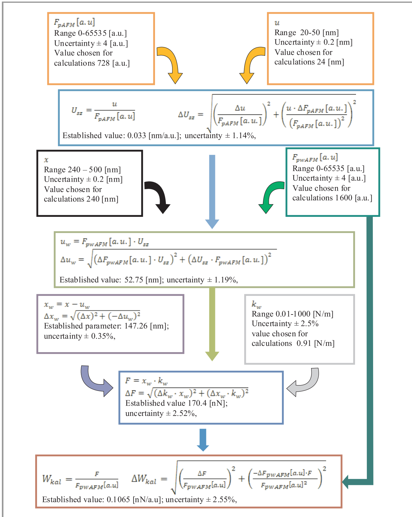
Fig. 4. Estimation of the uncertainty of the lateral force calibration method. Explanations: u – displacement of the cantilever tip during calibration procedure, F_{pAFM} – lateral force, U_{sz} – multiplier describing how big displacement of the cantilever tip causes a change of 1 a.u. of the lateral force during rigid/stiff sample test, F_{pwAFM} – change of the lateral force value, u_w – displacement of the cantilever tip during calibration on the calibration sample, x_w – real displacement, x – applied displacement, k_w – stiffness of the calibration sample, W_{kal} – calibration coefficient, F – lateral force in real units [nN].
