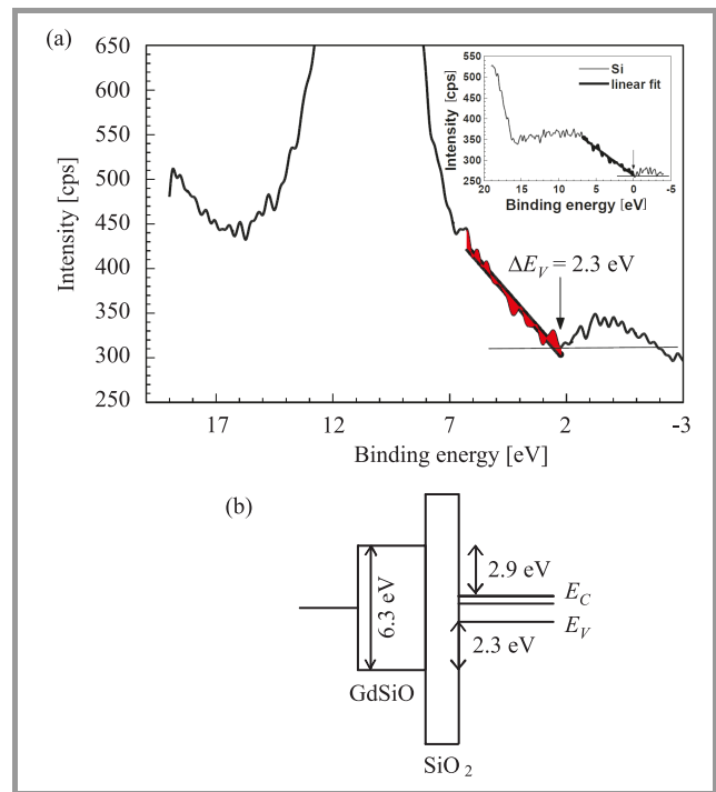
Fig. 6. (a) The XPS valence band spectrum and (b) the band diagram of ALD \text{GdSiO}/\text{SiO}_2/\text{Si}(100) structure.
