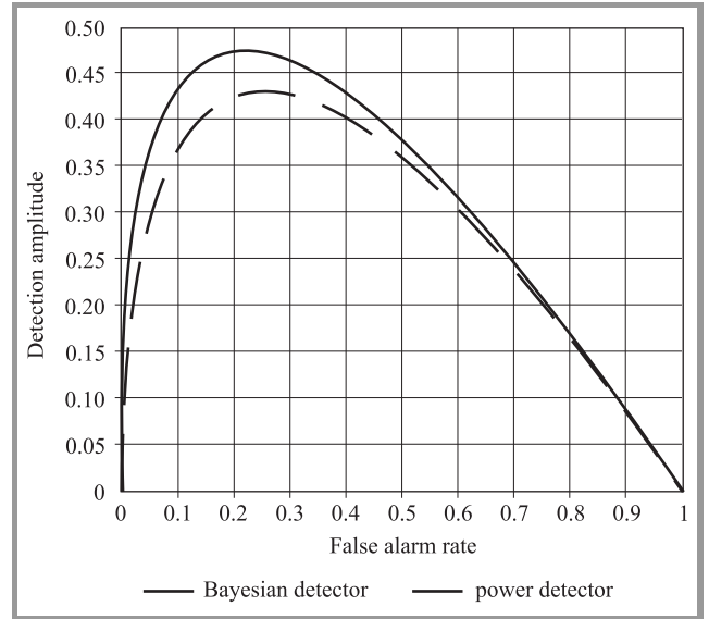
Fig. 1. Detection amplitude comparison in MIMO; M = 1 , N = 8 , L = 20 , \text{SNR} = -10 dB.
