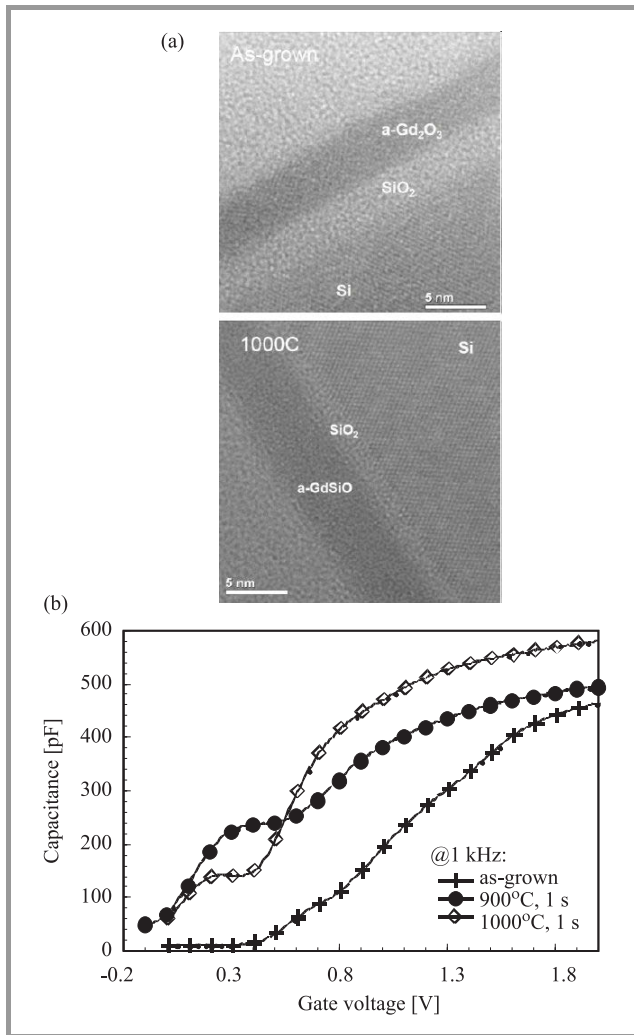
Fig. 1. (a) HRTEM images of \text{Gd}_2\text{O}_3/\text{SiO}_2 gate stacks as-deposited by ALD (top) and after RTA at 1000^\circ\text{C} for 1 s in \text{N}_2 (bottom); (b) C-V plots of corresponding MIS devices (Au/hi-k/ \text{SiO}_2/\text{Si}(100) ).
