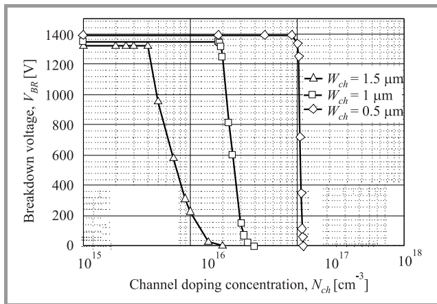
Fig. 6. Reverse blocking voltage, V_{BR} as a function of channel doping concentration, N_{ch} for N-on BGJFET with V_{th} = -10 V at 250°C.
