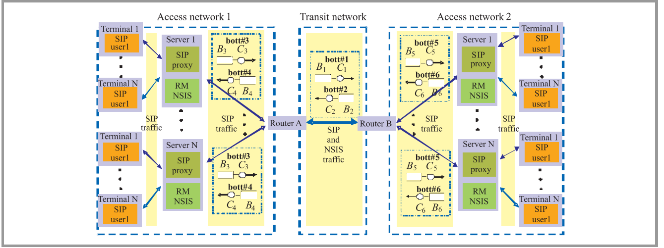
Fig. 10. Model of the EuQoS signaling system.
