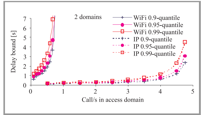
Fig. 6. Quantiles of T_{ti-td} for 2 WiFi or 2 IP domains versus \lambda_{ingress} ( \lambda_{ingress} = \lambda_{egress} = \lambda_{conf} ).
