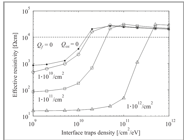
Fig. 16. Simulated effective resistivity values \rho_{eff} as a function of the trap density D_{it} for several fixed charges densities Q_{ox} and an applied bias value of 0 V.
