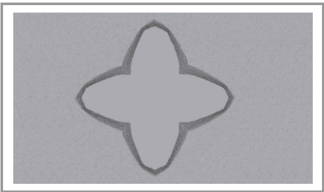
Fig. 9. Results of the simulations – using tuned Etch3D™ RPF parameters.
