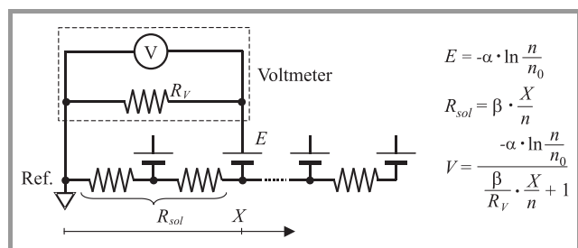
Fig. 10. A simple model of the \text{Cl}^- ion measurement setup using a number of cells.
