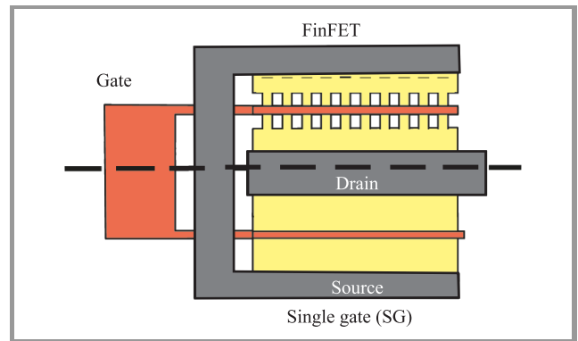
Fig. 7. Schematic top view of a FinFET composed of 10 fins (upper) and SG MOSFET (lower) occupying the same active silicon foot print.
