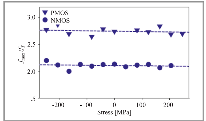
Fig. 13. Variation of (f_{max}/f_T) ratio with the applied mechanical stress for P- and NMOSFETs.
