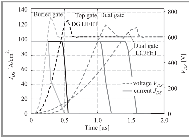
Fig. 15. A comparison of the switching characteristics of the N-off DGTJFET using the buried gate, the top gate and both gates with a N-off LCJFET with 10 \mu\text{m} cell pitch and double gate control. Turn-off in inductive circuit with R_G = 2 \Omega .
