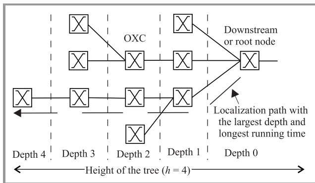
Fig. 3. Localization path tree.
