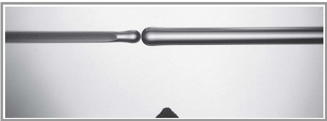
Fig. 6. Lens-tipped fibers positioned with \approx 10\text{ }\mu\text{m} gap (offset: 200\text{ }\mu\text{m} , loss: 5.48 dB).
