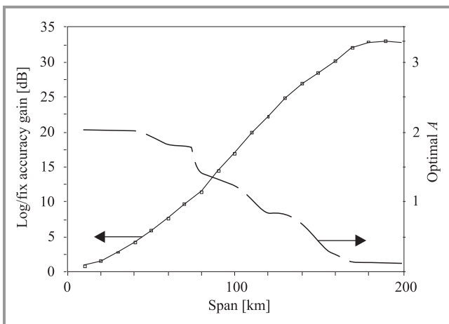
Fig. 6. Accuracy gain of logarithmic distribution over uniform one and optimal value of parameter A as a function of fiber span.
