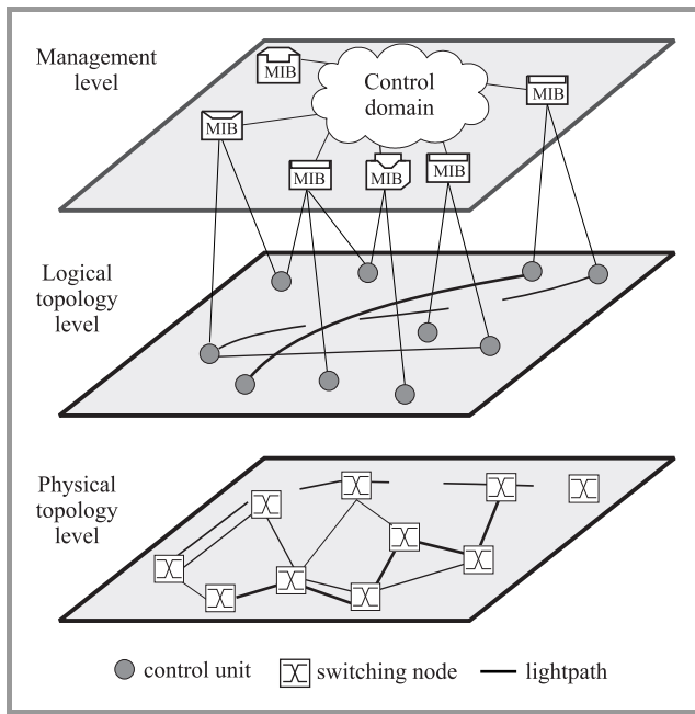
Fig. 2. The MIB distributed among element management systems.
