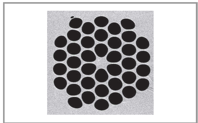
Fig. 2. Image of the cross section of the fibre taken by a scanning electron microscope.
