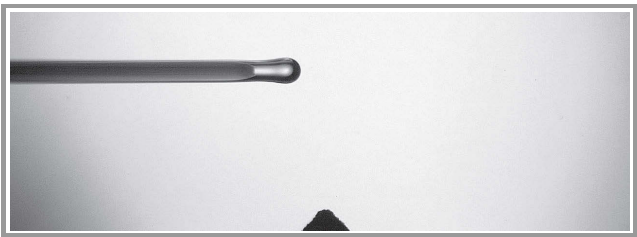
Fig. 5. PCF tip melted into a ball. Holes collapsed over 180\text{--}200\text{ }\mu\text{m} length.
