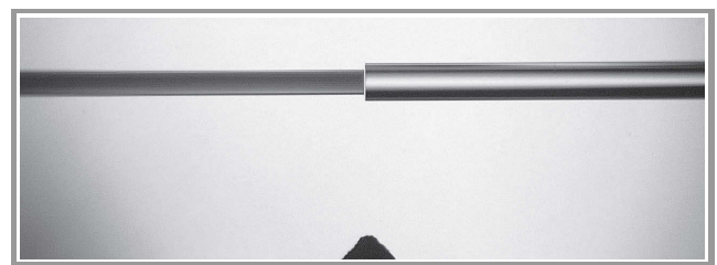
Fig. 2. Fibers cleaved and aligned with 10 \mu\text{m} gap (loss: 8.18 dB, electrode tip visible at the bottom).
