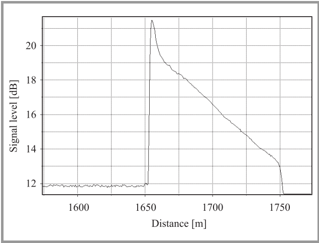
Fig. 16. OTDR trace of 104 m IPHT 282b4 preceded by 1645 m long SMF, \lambda = 1310 nm. Reflection spike is due to connector located between SMF and PCF.
