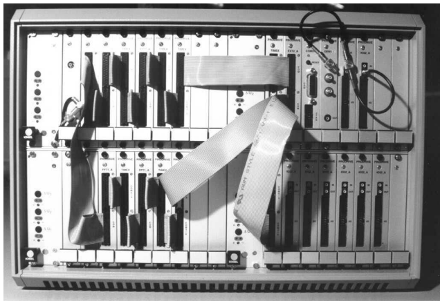
Fig. 3. Photograph of the computer system. The left upper quadrant contains the ADC and one pipeline of the spectrum processor. The second pipeline is placed in the left lower quadrant. The right upper quadrant contains the master processor and the linearisation module. The right lower quadrant contains the I/O modules for system control.
