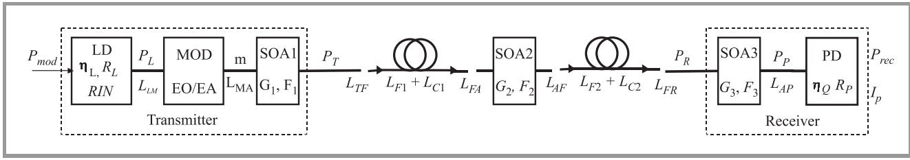
Fig. 5. Block diagram of the optical link.
