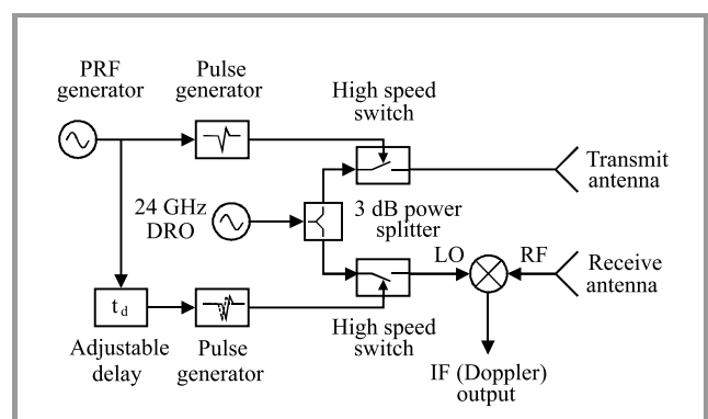
Fig. 1. Sensor block diagram. Explanations: IF – intermediate frequency, LO – local oscillator, PRF – pulse repetition frequency (in this case 4 MHz), RF – radio frequency, t_d – delay time, DRO – dielectric resonator oscillator.
