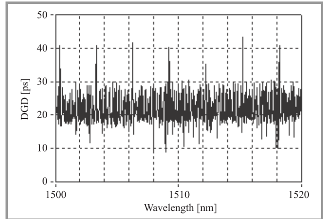
Fig. 16. DGD spectrum (IPHT Jena 252b5, fiber length 17.1 m, direction R-B, scan step 0.02 nm).
