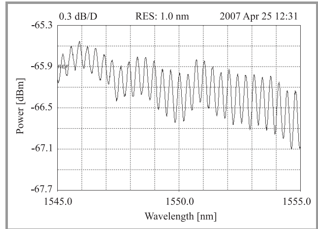
Fig. 15. Transmission spectrum in FA measurement (IPHT Jena 252b5, length 17.1 m).
