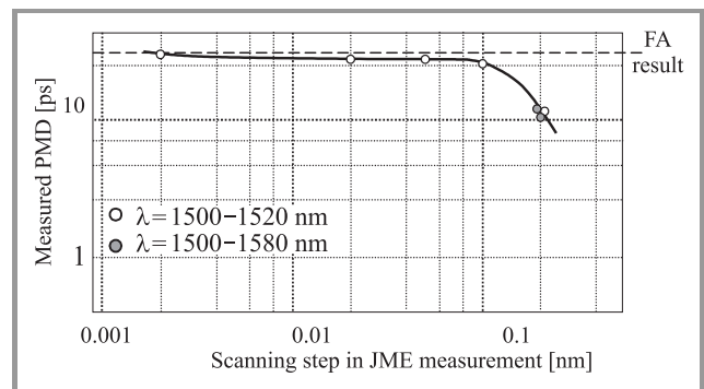
Fig. 17. Comparison of JME and FA measurements (IPHT Jena 252b5, length 17.1 m).
