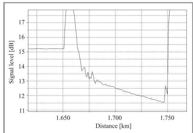
Fig. 5. OTDR trace of Yb1200-10/125DC-PM fiber with SMF pigtail, connected to 1650 m of SMF ( \lambda = 1310\ \text{nm} , pulse width 50 ns).
