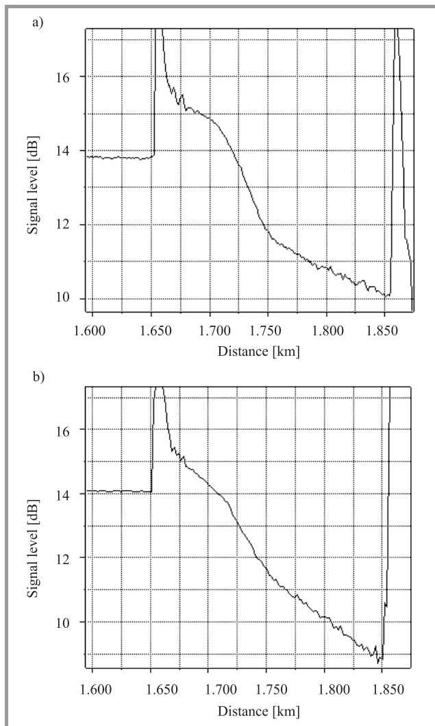
Fig. 4. OTDR traces of Yb1200-6/125DC fiber with SMF pigtail, connected to 1650 m of SMF: (a) \lambda = 1310\ \text{nm} ; (b) \lambda = 1550\ \text{nm} .
