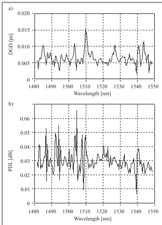
Fig. 8. DGD (a) and PDL (b) spectra (Liekki Yb1200-6/125DC, length 200 m).
