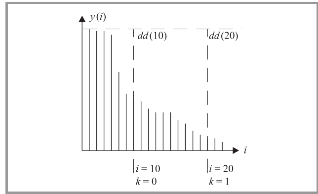
Fig. 2. Example of distances set division.
