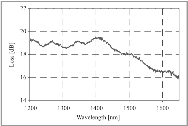
Fig. 3. Spectral loss of 1 m IPHT Jena 252b5 PCF spliced to 2 m long SMF pigtails.
