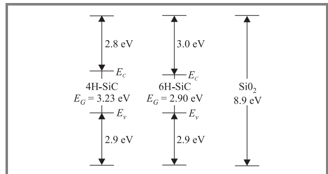
Fig. 2. Band offset of 4H- and 6H-SiC in comparison to silicon dioxide [3].
