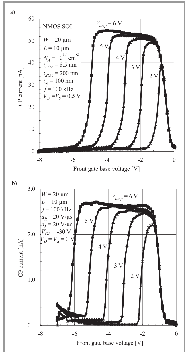
Fig. 3. Front-interface CP current as a function of front-gate base voltage with gate voltage amplitude as a parameter: (a) N_{body} = 10^{17} cm ^{-3} ; (b) N_{body} = 10^{18} cm ^{-3} , annealed.
