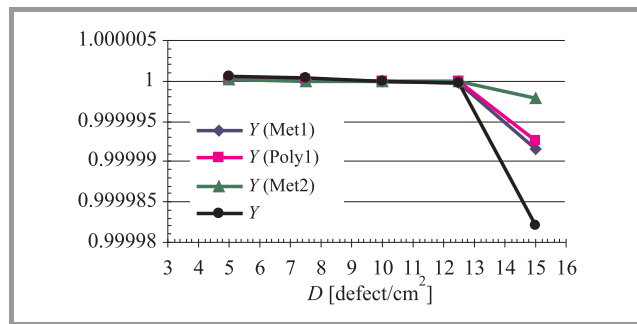
Fig. 8. Defect-related yield normalized to that obtained at nominal value of parameter D ( X = 20\% , p = 3 ).
