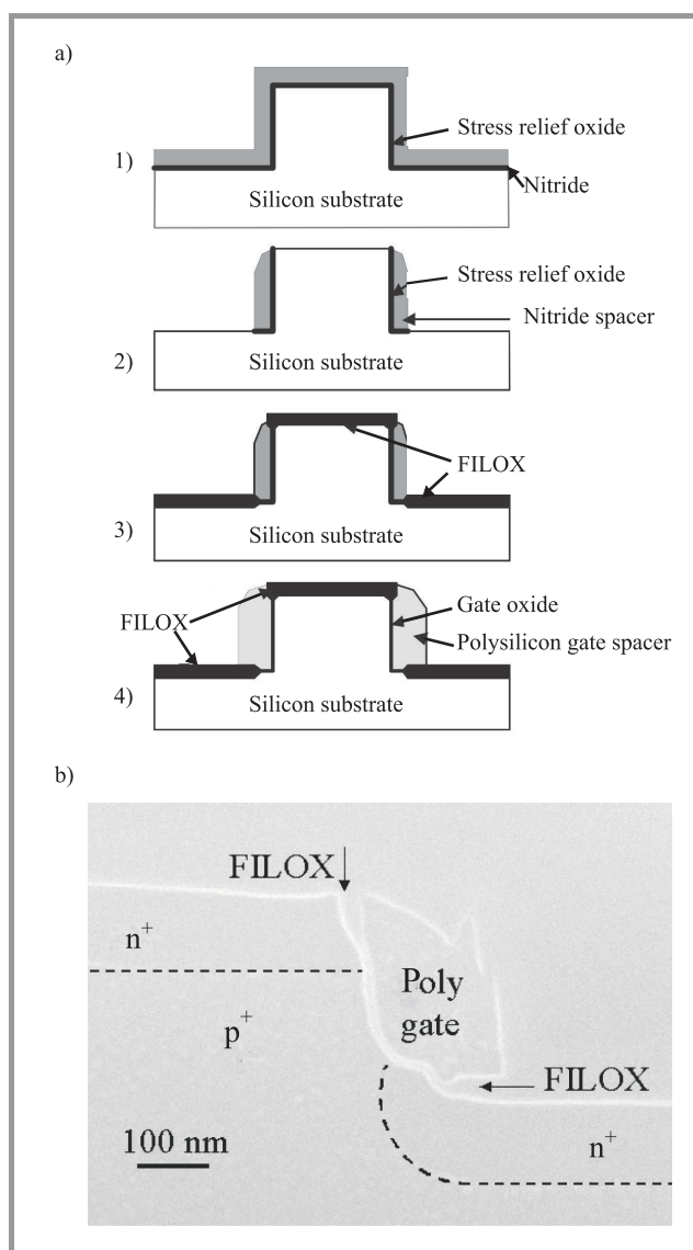
Fig. 1. Vertical MOSFET: (a) process flow and schematic cross-section of a FILOX; (b) photo of the device.
