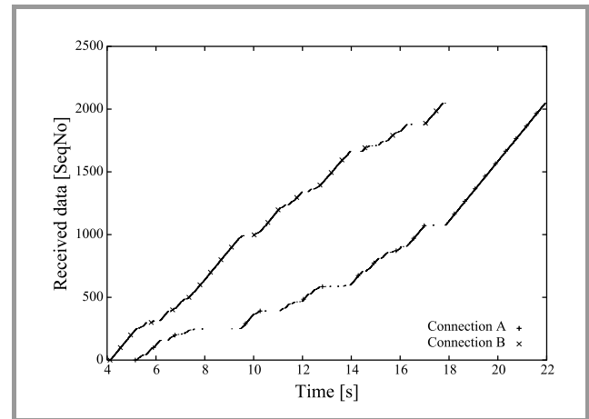
Fig. 9. Hybrid model – controlled SNR.
