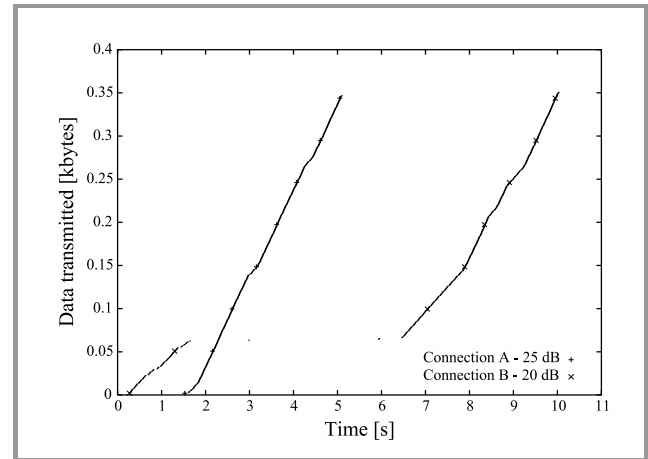
Fig. 2. Stationary SNR, RTS/CTS enabled.
