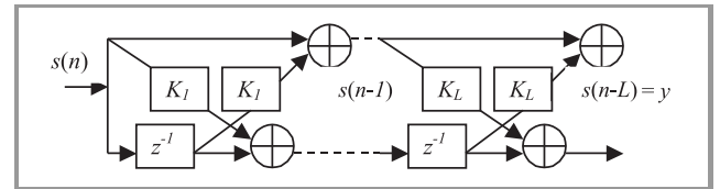
Fig. 4. A structure of whitening lattice filter (see Appendix A).
