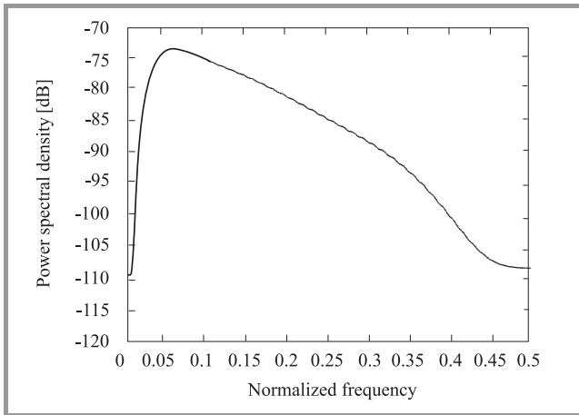
Fig. 3. Noise power spectral density.
