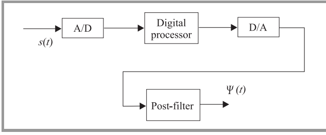
Fig. 7. Hybrid filter.
