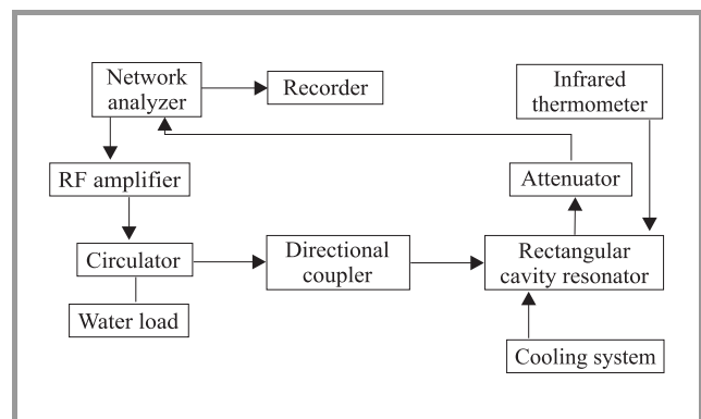
Fig. 6. Measuring system.
