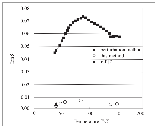
Fig. 12. \tan\delta versus temperature of PET.
