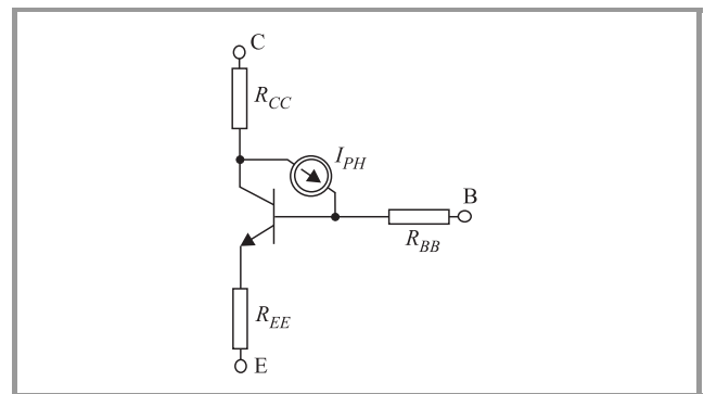
Fig. 19. Simplified SPICE-based HBT phototransistor model.
