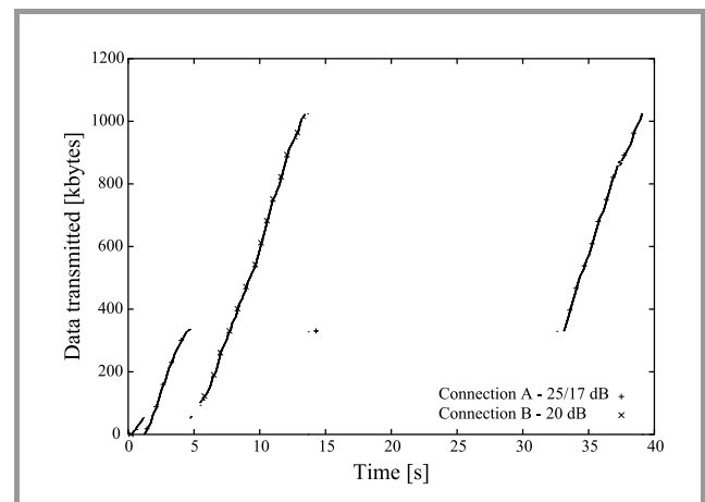
Fig. 3. Controlled SNR, RTS/CTS enabled.
