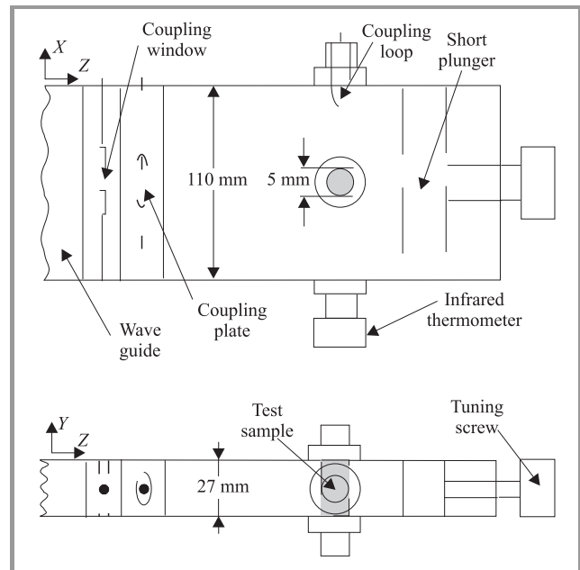
Fig. 5. TE_{102} mode rectangular cavity resonator.
