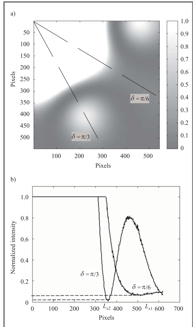
Fig. 4. Overexposed far field intensity distribution (a); cross sections for two angles \delta = \pi/6 and \delta = \pi/3 (b). LMA-10 fiber, z = 22 \text{ mm} , \lambda = 670 \text{ nm} .
