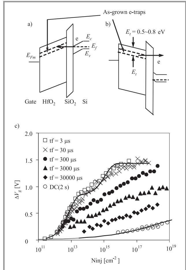
Fig. 4. Energy band diagrams of as-grown e-traps in \text{HfO}_2 . (a) e trapping at V_g > 0 V. (b) e detrapping at V_g < 0 V. (c) Dynamic behavior of electron trapping measured by different techniques. The data represented by symbol “o” was measured by the traditional DC I_d - V_g with V_g increasing with a step of 0.1 V for each point. The data in other symbols were obtained by the pulsed I_d - V_g technique [18].
