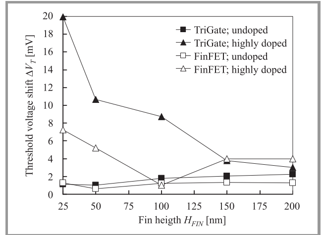
Fig. 13. \Delta V_T versus fin height H_{FIN} for FinFET and triple-gate structures with low ( N_A = 10^{15} \text{ cm}^{-3} ) and high ( N_A = 10^{18} \text{ cm}^{-3} ) body doping. W_{FIN} = 50 nm, L_G = 500 nm.
