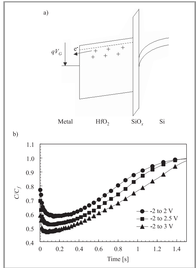
Fig. 6. (a) Energy band diagram showing positive charges are generated by electrons detrapping from pre-existed oxide defects. (b) Capacitance-transient curves of an HfO 2 sample showing undershoots [20].
