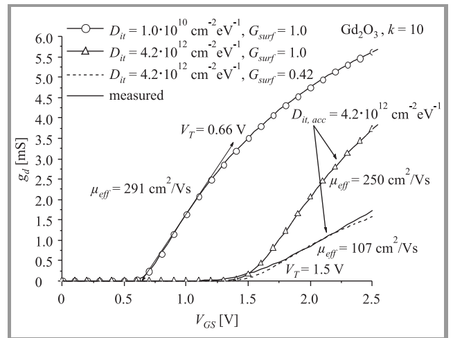
Fig. 10. Comparison of channel conductivities, threshold voltages and carrier mobility of measured data and simulated curves of \text{Gd}_2\text{O}_3 -devices illustrating the effect of ideal and degraded interfaces by simulation.
