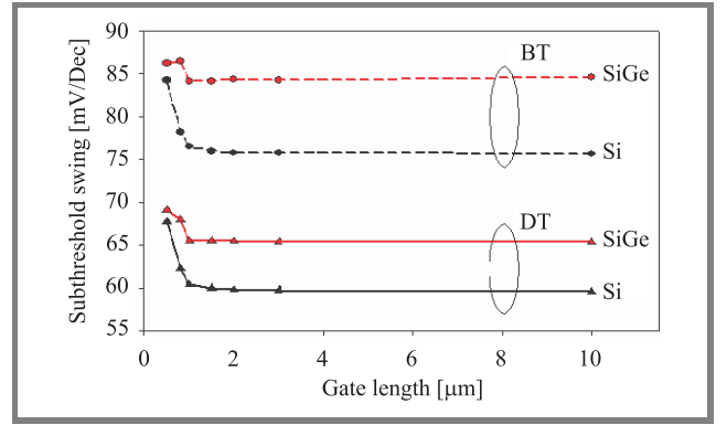
Fig. 8. Subthreshold swing in body tied and dynamic threshold modes as a function of gate length.
