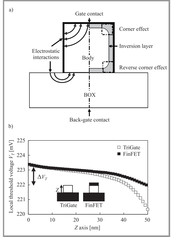
Fig. 12. (a) Cross-section of a triple-gate structure showing the electrostatic interactions leading to corner effects. (b) Local threshold voltage along the vertical channel for low doped ( N_A = 10^{15} \text{ cm}^{-3} ) FinFET and triple-gate FET with W_{FIN} = 50 nm, H_{FIN} = 50 nm, and L_G = 0.5 \mu\text{m} .
