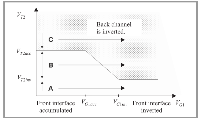
Fig. 8. The relationship between the threshold voltage of the back channel ( V_{T2} ) and the front-gate voltage ( V_{G1} ) by the model of Lim and Fossum. When the front interface is accumulated ( V_{T1acc} ), the threshold voltage of the back channel becomes constant. When the back gate is in region A and the front gate is swept, only the front channel is inverted. When the back gate is in region B and the front gate is swept, the back channel is turned off and on by the front gate voltage. When the back gate is in region C and the front gate is swept, the back channel cannot be turned off by the front gate voltage because of the accumulation layer at the front interface.
