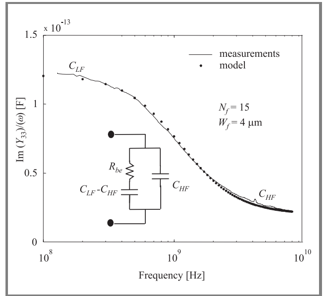
Fig. 6. Measured and simulated \text{Im}(Y_{33})/(\omega) data as a function of frequency for V_g = V_b = 0.6 V and V_d = 1.2 V, inset: R-C model used.
