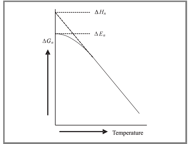
Fig. 2. Temperature dependence of the free energy position, \Delta G_n of an interface trap often occurring in semiconductors [19]. For not too low temperatures, \Delta G_n(T) approaches a linear function. As the entropy is \Delta S_n = -\partial(\Delta G_n)/\partial T , this quantity is temperature independent for the higher temperatures. At T = 0 , the free energy and the eigen energy coincide. In an activation measurement, where the slope of an Arrhenius plot is \Delta H_n , this quantity is the extrapolated value of \Delta G_n in the temperature interval where the measurement is made. For simplicity, in the present treatment, we assume that \Delta G_n is linear down to T = 0 , which makes \Delta G_n = \Delta H_n = \Delta E_n at this temperature.
