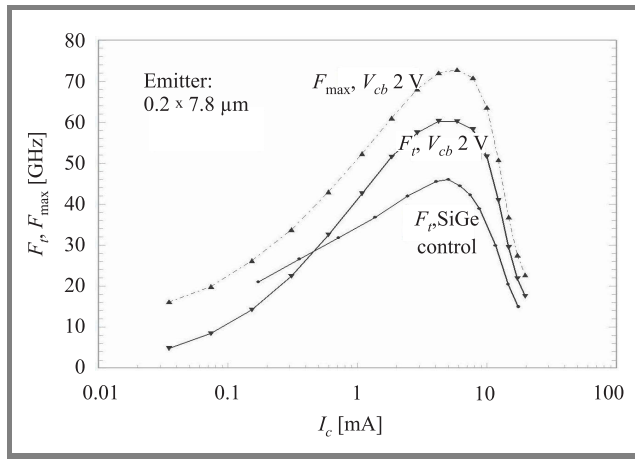
Fig. 11. Effect of a 150 keV, 5 \cdot 10^{14} \text{ cm}^{-2} \text{ F}^+ implant on the f_T and f_{\max} of a double polysilicon silicon bipolar transistor. After Kham et al [15] © IEEE.
