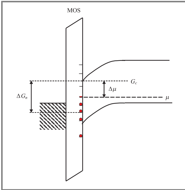
Fig. 1. Band model of the MOS structure on a free energy scale.
