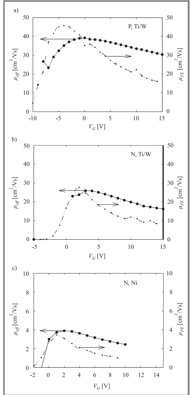
Fig. 5. Channel mobility extracted from the output characteristics of single hexagonal cell devices with P implanted source and Ti/W contact (a), with N implanted source and Ti/W contact (b) and with N implanted source and nickel silicide contact (c). Channel length L_{ch} = 2 \mu\text{m} .
