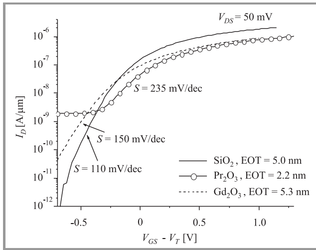
Fig. 8. Measured sub-threshold characteristics of fabricated \text{Pr}_2\text{O}_3 -, \text{Gd}_2\text{O}_3 - and \text{SiO}_2 devices.
