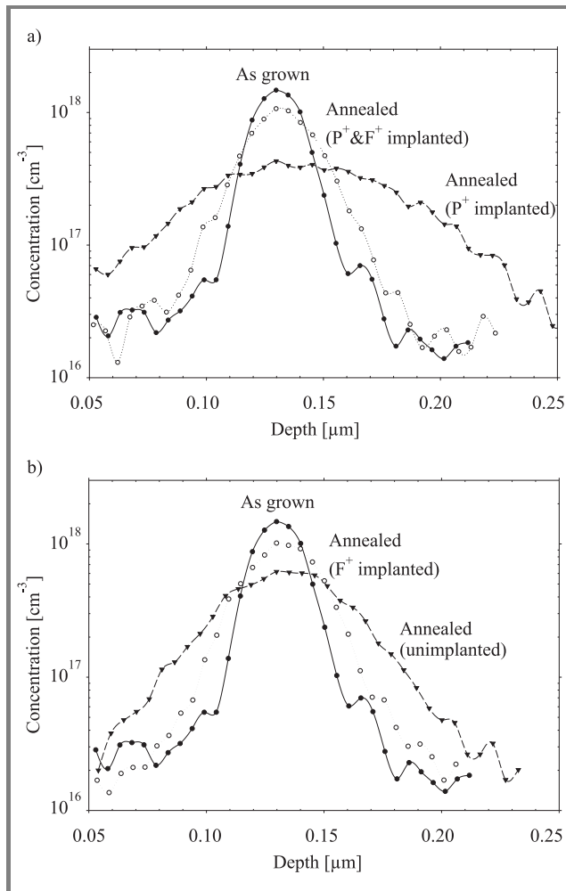
Fig. 7. Boron SIMS profiles of a buried marker layer after anneal for 30 s at 1000^\circ\text{C} in nitrogen: (a) samples implanted with \text{P}^+ only and with \text{P}^+ and \text{F}^+ ; (b) an unimplanted sample and a sample implanted with \text{F}^+ only. After Mubarek et al. [9] © AIP.
