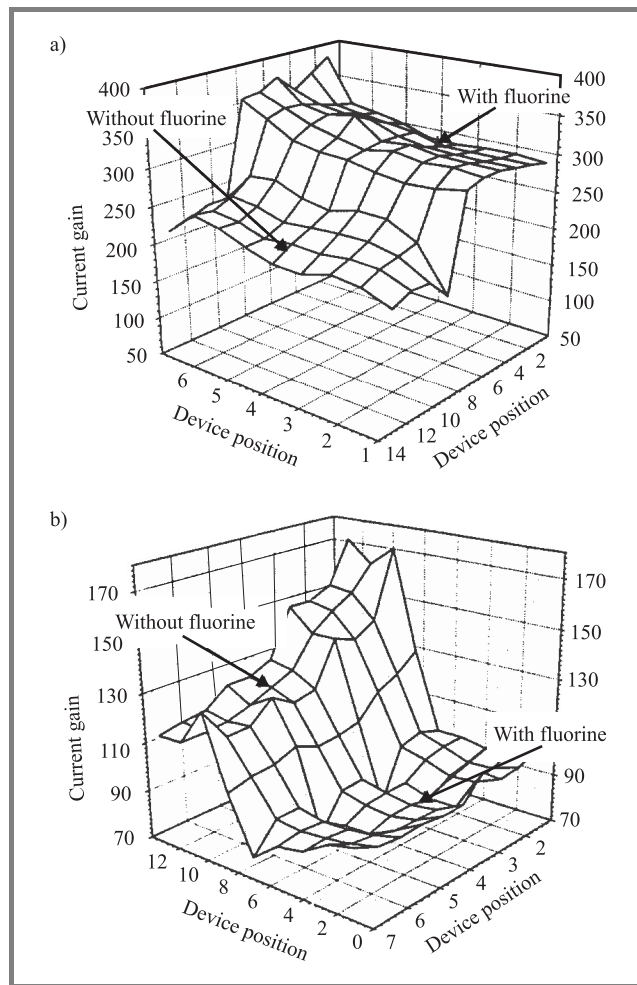
Fig. 1. The 3D plot of polysilicon emitter bipolar transistor gain measured across a wafer. The wafer had a 50 keV, 1 \cdot 10^{16} \text{ cm}^{-2} \text{F}^+ implant into half of each wafer and the wafers were given the following anneals: (a) 15 min at 850°C; (b) 120 min at 850°C. After Moiseiwitsch et al. [4] © IEEE.
