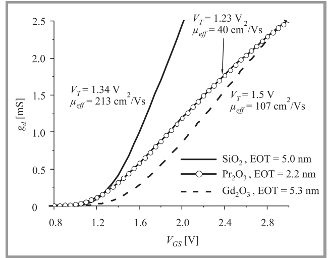
Fig. 9. Measured transconductance and extracted mobility values of fabricated \text{Pr}_2\text{O}_3 -, \text{Gd}_2\text{O}_3 - and \text{SiO}_2 devices.
