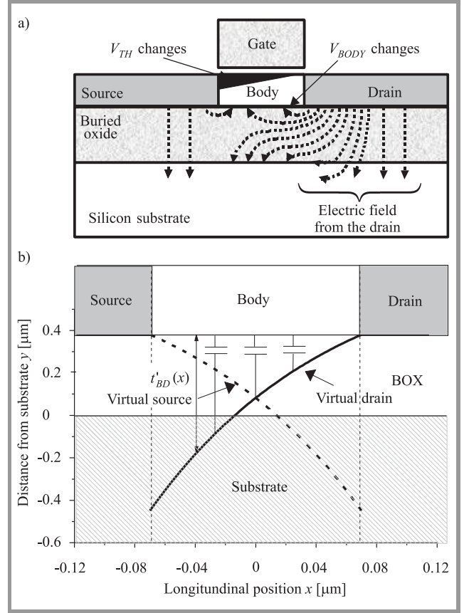
Fig. 17. (a) Schematics of the fringing fields leading to DIVSB effect and (b) equivalent representation of buried oxide fringing capacitances and source/drain virtual electrodes.
