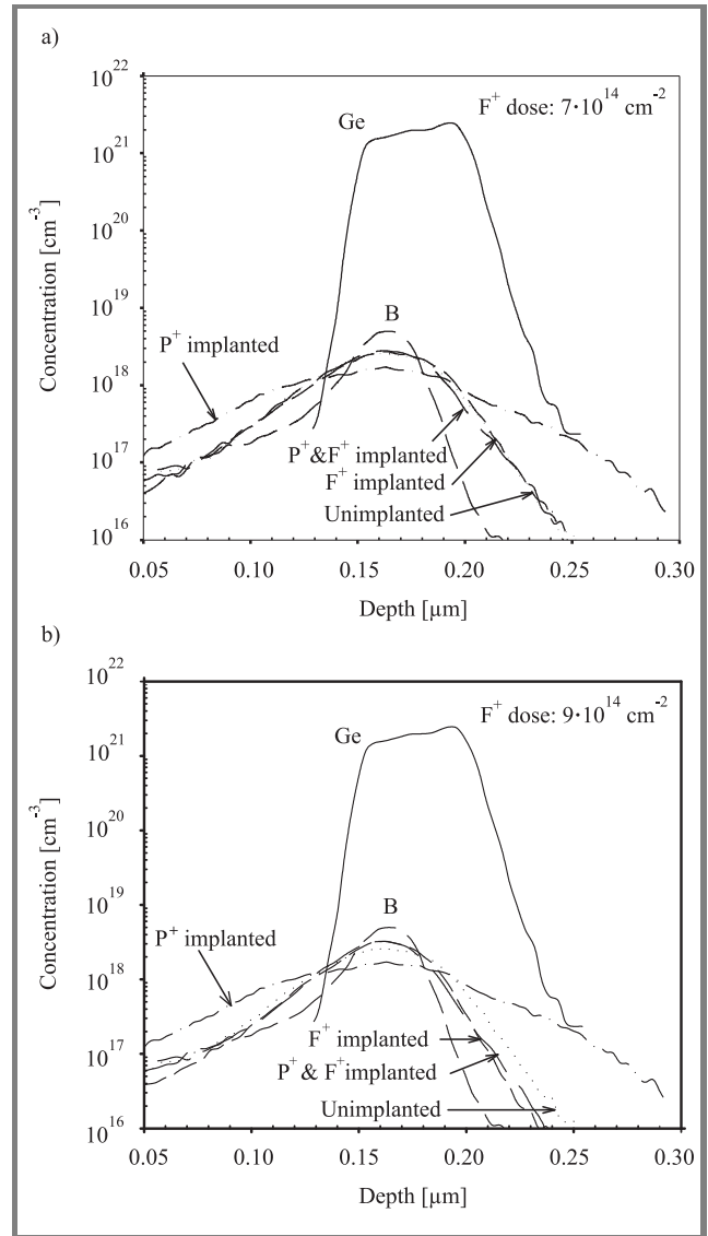
Fig. 8. Boron profiles after anneal for 30 s at 1000^\circ\text{C} in nitrogen for samples implanted with \text{P}^+ and \text{F}^+ , \text{P}^+ only, \text{F}^+ only and for an unimplanted sample. Results are shown for \text{F}^+ implantation doses of (a) 7 \cdot 10^{14} \text{ cm}^{-2} and (b) 9 \cdot 10^{14} \text{ cm}^{-2} . After Mubarek et al. [12] © IEEE.
