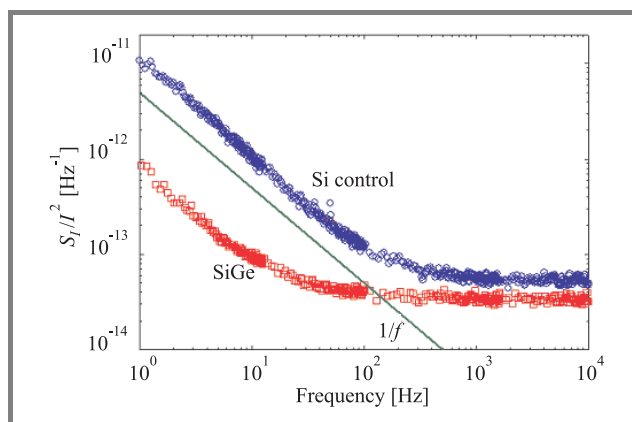
Fig. 3. Current noise power spectral density, demonstrating that SiGe devices display lower noise than Si control ( V_{GT} = -3.5\ \text{V} , L = 40\ \mu\text{m} , W = 40\ \mu\text{m} , T = 300\ \text{K} , V_{DS} = -50\ \text{mV} ) [1].
