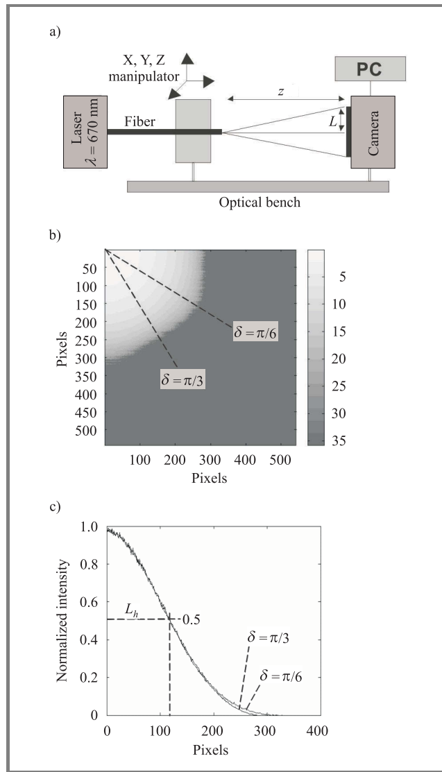
Fig. 3. Far field arrangement (a); normal far field intensity distribution – logarithmic scale (b); cross sections for two angles \delta = \pi/6 and \delta = \pi/3 (c). LMA-10 fiber, z = 22 \text{ mm} , \lambda = 670 \text{ nm} .
