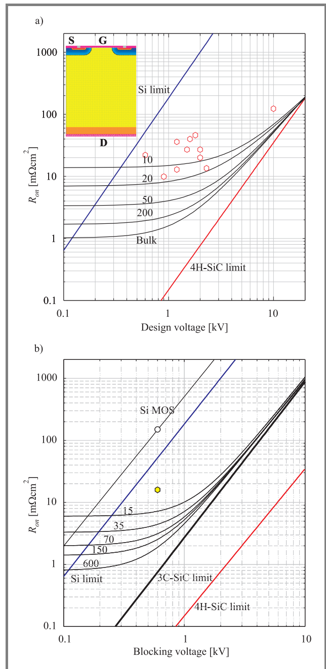
Fig. 10. A comparison of calculated and experimental data for 4H-SiC (a) and the 3C-SiC (b) DMOSFETs, respectively. The calculated data are for the ideal structure with 10\ \mu\text{m} cell pitch and 1\ \mu\text{m} channel length (the 1\ \mu\text{m} line-width lithography) and for different values of channel mobility. The experimental data point for 3C-SiC corresponds to the structure with 28\ \mu\text{m} cell pitch and 2\ \mu\text{m} channel length ( R_{on} = 17\ \text{m}\Omega\text{cm}^2 ). The experimental values for 4H-SiC are values published by others.
