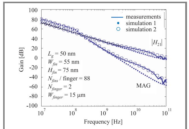
Fig. 9. Measured and simulated |H_{21}| and maximum available gain (MAG) for a RF FinFET. The models considered were a classical equivalent circuit for FET (simulation 1, dots) and that of Fig. 10 (simulation 2, circles).
