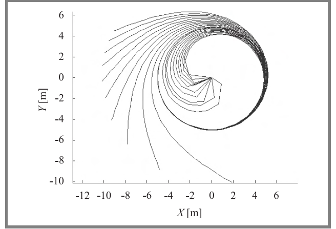
Fig. 3. Trajectories of two object formation member in the motion plane with different initial parameters.
