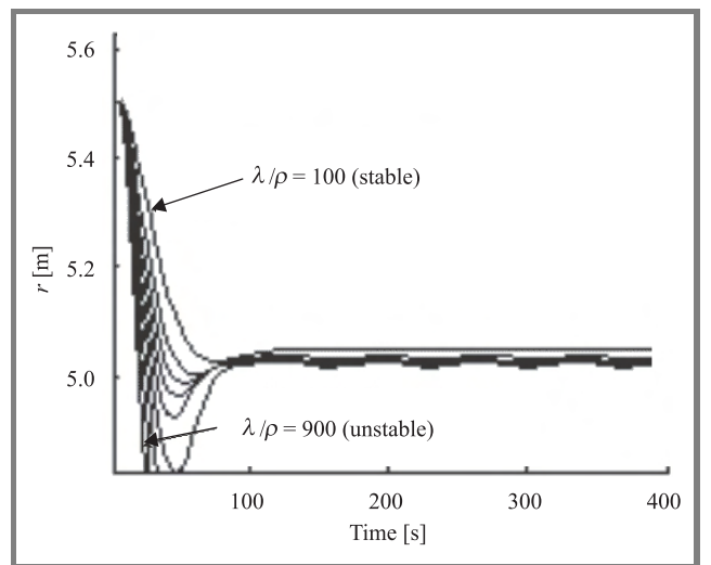
Fig. 5. Radial distance changes in time for different \lambda/\rho values (2 objects formation).
