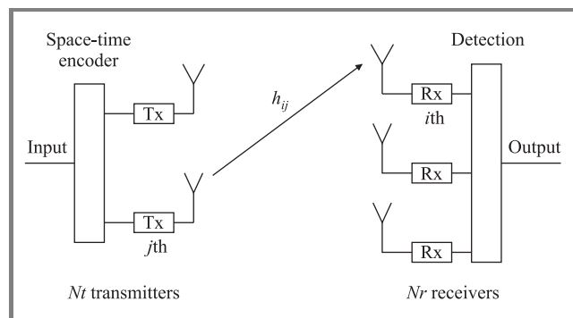
Fig. 1. Block diagram of MIMO system.
