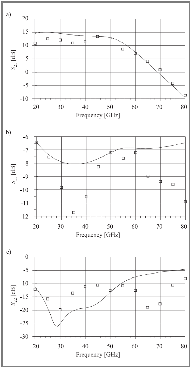
Fig. 5. Simulated and measured: (a) power gain ( V_{CC} = 4 V); (b) input return loss; (c) output return loss.
