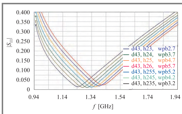
Fig. 7. |S_{11}| for several different dimension configurations.
