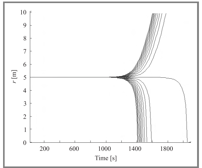
Fig. 4. Distance changes from common mass center for two object formation member with different initial parameters.
