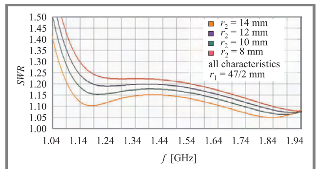
Fig. 5. SWR for LM113 output with cardioid coupling part.
