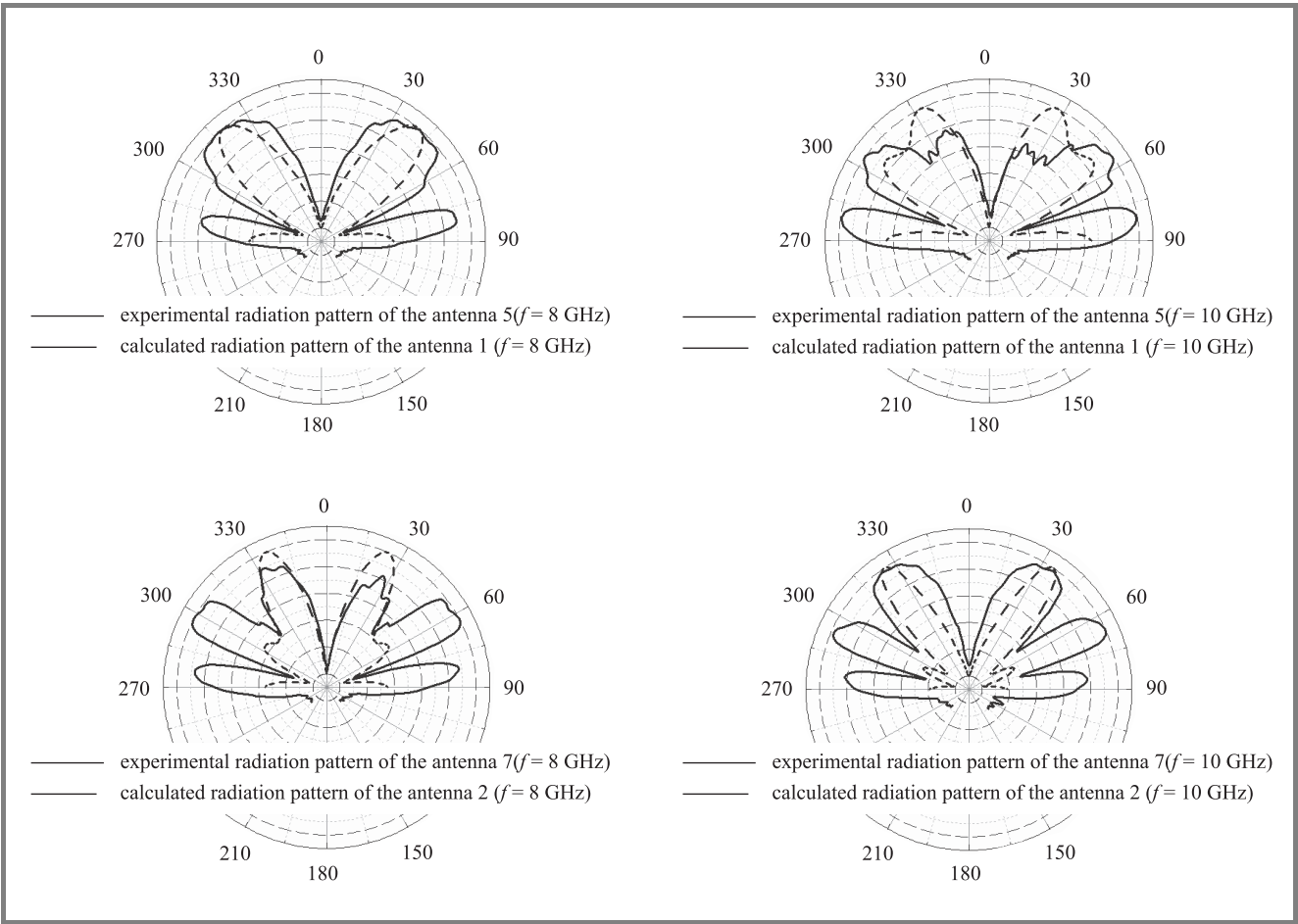
Fig. 6. Radiation patterns of some antenna designs.
