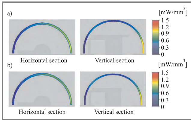
Fig. 6. Average dissipated power density, cardioid: (a) r_2 = 8 mm and (b) r_2 = 14 mm.
