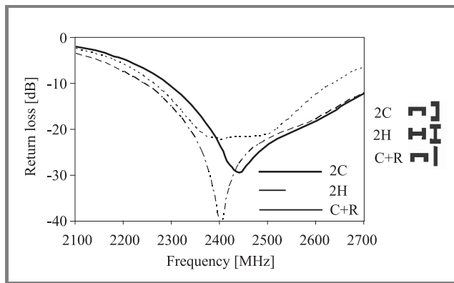
Fig. 3. Simulated return loss characteristics for antennas fed with a various pairs of slots (2C, 2H, C+R).
