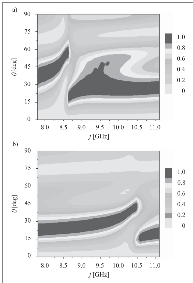
Fig. 2. Calculated radiation patterns normalized at the every fixed frequency: (a) antenna N1; (b) antenna N2.
