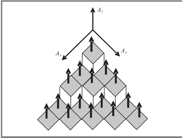
Fig. 4. Entire probability states in 3D plain for twice BW of A_z traffic ( n = 4 ).
