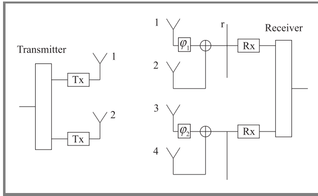
Fig. 2. MIMO system incorporating phased array antennas in each receiver branch ( \phi – phase shifter, antenna spacing: \lambda in transmitter, \lambda/2 in receiver).
