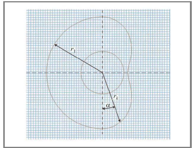
Fig. 4. Coupling disc of cardioid shape.
