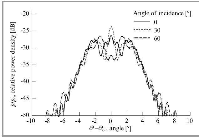
Fig. 16. Radiation pattern in a distance r = 150 m of a spherical reflector ( D_x = D_y = 0.7 m, h = 0.006 m) with infinite conductivity and for different angles of incidence \Theta_0 .
