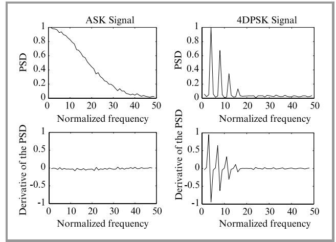
Fig. 1. PSD and its derivative ( \nu = 200 Bd; SNR = 15 dB).
