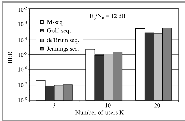
Fig. 6. BER versus users number, N = 127 , E_b/N_0 = 12 dB.
