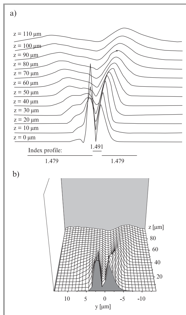
Fig. 2. Spatial transient process of the radiation field propagation simulated by the FFT-BPM (a) and by the FD-BPM (b).
