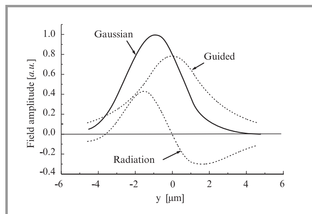
Fig. 1. Input Gaussian beam profile, its modal and radiation parts.
