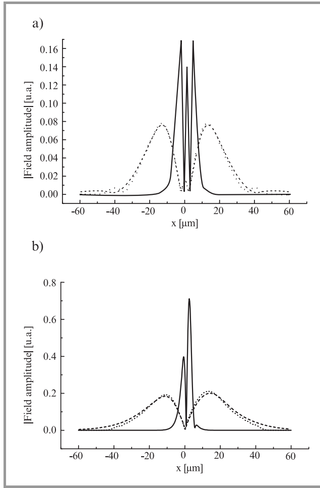
Fig. 3. Transverse distributions of the radiation field at the input endface of the waveguide (solid line), and after the distance of 150 \mu\text{m} , simulated by the FFT-BPM (dashed line) and the FD-BPM (dotted line), respectively. (a) Symmetric excitation (shift = 0), (b) asymmetric excitation (shift = 2 \mu\text{m} ).
