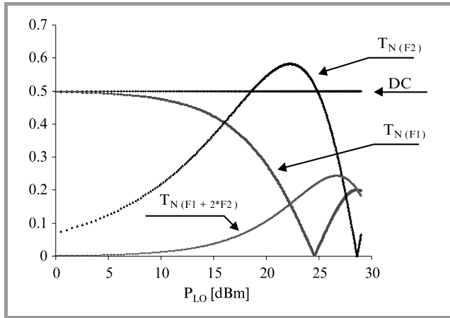
Fig. 4. Products of optical-microwave mixing for circuit shown in Fig. 3 and at bias in the inflexion point. Calculations have been made for Z_0 = 50 \Omega and V_\pi = 7 V.
