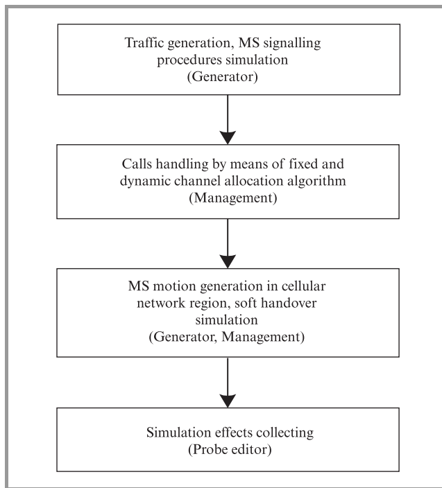
Fig. 2. Simulation program structure.
