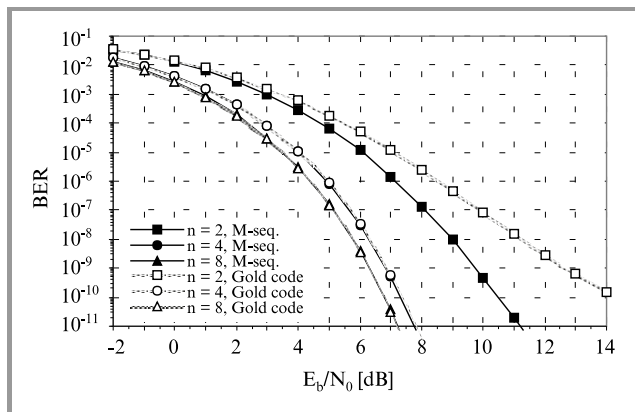
Fig. 7. Simulation results for Walsh mapping, M = 64 , K = 10 , added M- and Gold sequences spreading.
