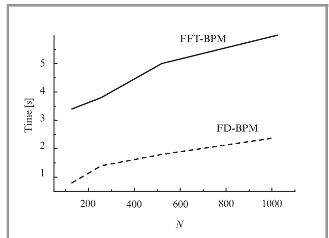
Fig. 5. Calculation time of the numerical simulations of the radiation field propagation (distance = 150 \mu\text{m} , \Delta z = 0.5 \mu\text{m} ), using the FD-BPM and the FFT-BPM, depending on the number of grid points.
