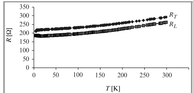
Fig. 9. Low-temperature resistance of recrystallized poly-Si resistors with N = 1.7 \cdot 10^{20} \text{ cm}^{-3} . R_T and R_L represent transversal and longitudinal resistance as related to the laser scan direction.
