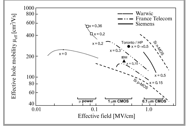
Fig. 2. Available experimental data on 300 K hole effective mobilities obtained in pseudomorphic \text{Si}/\text{Si}_{1-x}\text{Ge}_x/\text{Si} structures plotted against effective field ( E_{\text{eff}} ), all data refer to buried SiGe channels except for the IBM sample where the gate dielectric was produced by plasma oxidation. The alloy composition in the Toronto/HP sample was graded. The squares refer to modulation-doped structures. The bars indicate the range of E_{\text{eff}} values present in micropower, 1 and 0.1 \mu\text{m} CMOS technologies. \beta is usually taken as 3 for holes [6], in order to obtain an universal curve independent of doping specifications. That practice is followed here, but we note that this tends to over-emphasise the superiority of the electron channel where \beta is chosen as 2.
