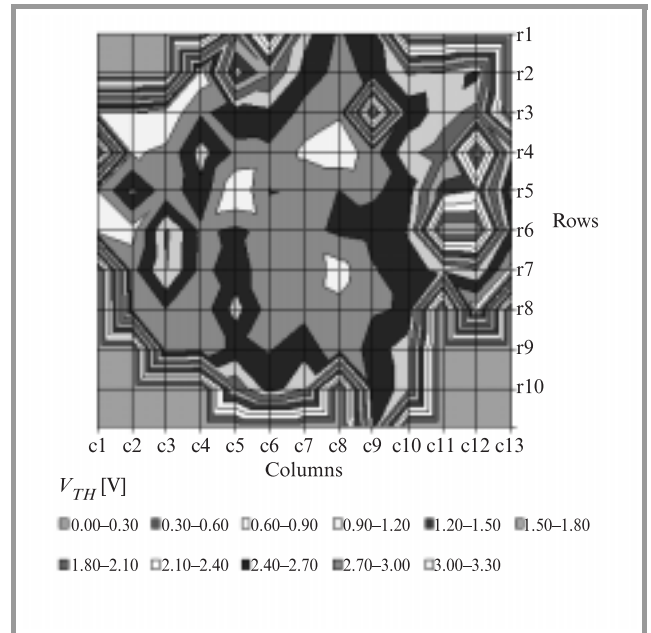
Fig. 8. 3D distribution map of the threshold voltage V_{TH} value variations over the substrate's surface.
