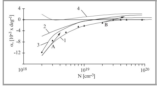
Fig. 4. Calculated TCR of poly-Si resistors near 20°C for L = 120 \text{ nm} and 2 - L = 1 \mu\text{m} , compared with 3 – simulation and experimental data from [5] (triangles). Curve 4 corresponds to the data for bulk silicon.
