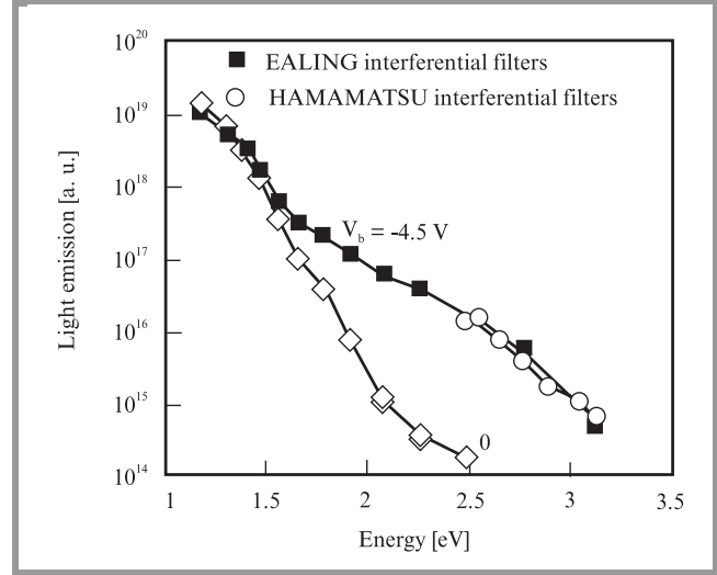
Fig. 4. Impact of the substrate bias on the light emission for deep submicron bulk MOSFETs.
