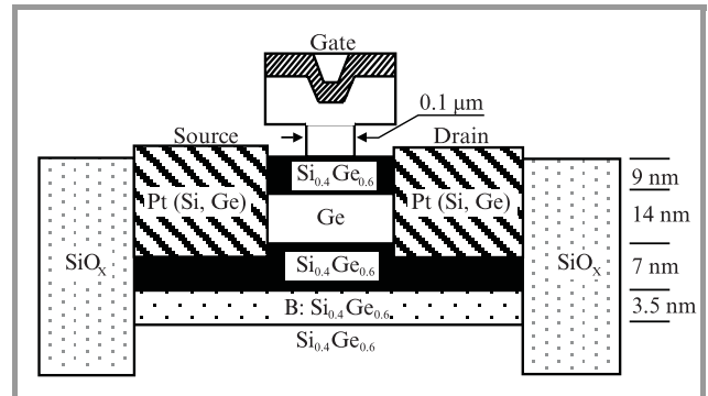
Fig. 16. 0.1 \mu m gate length strained Ge p-MODFET. Contact pad metallisation not shown (after Hammond et al. [26]).
