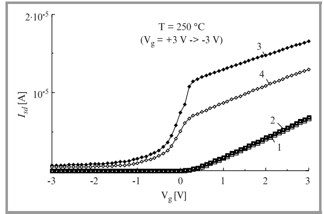
Fig. 12. Source-drain current versus gate voltage in dependence on conditions of the substrate: (1) V_{bg} = -30 V, hold time is 0 s; (2) V_{bg} = -30 V, hold time is 150 s; (3) V_{bg} = -0 V, hold time is 0 s after stressing at V_{bg} = -30 V for 150 s; (4) V_{bg} = 0 V, hold time is 150 s.
