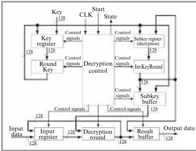
Fig. 9. The decryption unit.
