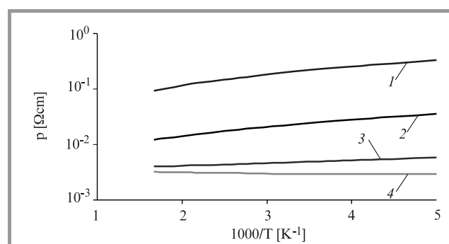
Fig. 1. Calculated p-type poly-Si resistivity versus temperature for carrier concentration N = 1.3 \cdot 10^{20} \text{ cm}^{-3} and the following values of the average grain size: 1 – 100 nm; 2 – 1 \mu\text{m} ; 3 – 10 \mu\text{m} ; 4 – 100 \mu\text{m} .
