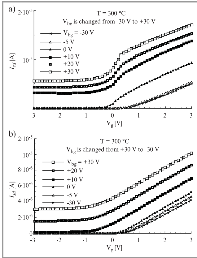
Fig. 10. Source-drain current versus gate voltage for different substrate voltages ( V_{bg} ) at 300^\circ\text{C} when substrate voltage is swept from -30 V to +30 V (a) and from +30 V to -30 V (b).
