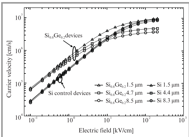
Fig. 14. Carrier velocity versus horizontal field, extracted from measurements on thick oxide (140 nm) Si_{0.8}Ge_{0.2} p-MOSFETs and by comparison with a drift diffusion model (after Kaya et al. [17]).
