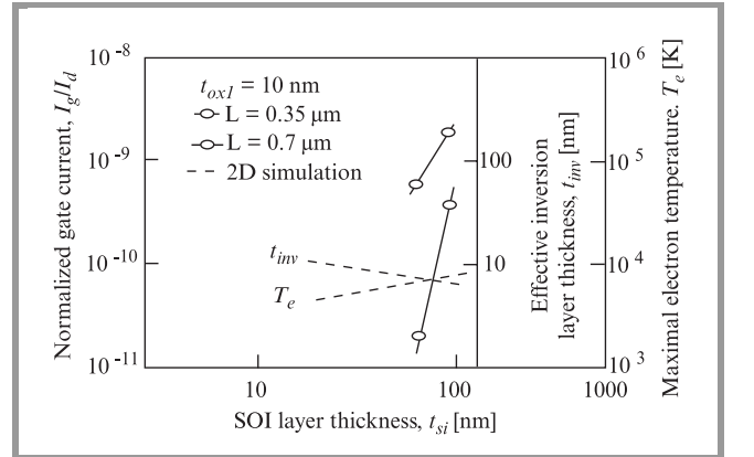
Fig. 13. Comparison between the variations of the normalized gate current, the inversion layer thickness and the electron temperature versus Si film thickness for fully depleted SOI MOSFETs.
