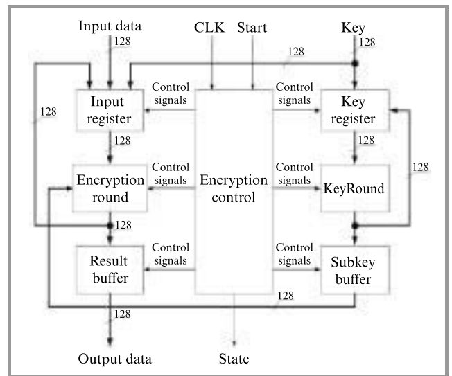
Fig. 8. The encryption unit.
