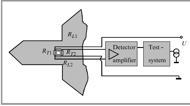
Fig. 2. Electrical scheme of the piezoresistive cantilever measurement system.
