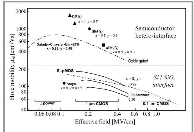
Fig. 3. Available experimental data on 300 K hole mobilities obtained in compressively strained \text{Si}_{1-x}\text{Ge}_x and tensile strained Si grown on virtual substrates with terminating composition structures \text{Si}_{1-x}\text{Ge}_x . The upper section shows mobilities for remote doped hetero-interfaces and the lower section refers to oxide-gate/(tensile strained) Si interfaces. I denotes „inverted” and N denotes „normal” interface. The oxide-gated data refer to inversion layers. \beta = 3 .
