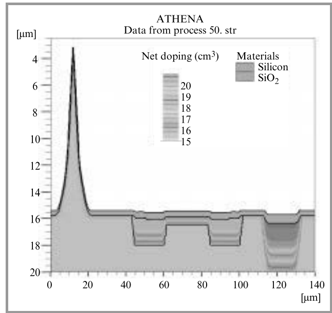
Fig. 8. Cross-sections of the piezoresistive cantilever – piezoresistors diffusion.
