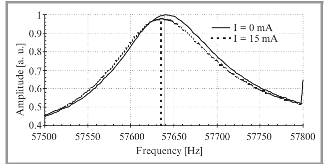
Fig. 8. Shift in the cantilever resonance frequency due to the power supplied to the microheater.
