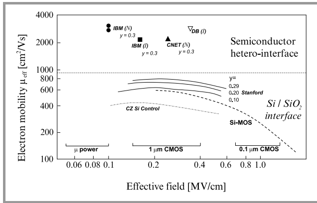
Fig. 1. Available experimental data on 300 K electron mobilities in strained Si grown on virtual substrates with terminating composition \text{Si}_{1-x}\text{Ge}_x versus the effective field E_{\text{eff}} [2, 3]. E_{\text{eff}} = \frac{e}{\epsilon_s} [N_{\text{depl}} + \frac{1}{\beta} n_s] where \epsilon_s is the absolute permittivity of Si, N_{\text{depl}} is the depletion charge density, and n_s is the carrier density. The upper section shows mobilities at remote doped hetero-interfaces and the lower section refers to oxide-gate/(tensile strained) Si interfaces. I denotes „inverted” modulation-doped structure (doping supply layer below strained silicon) and N denotes „normal” interface case (doping above silicon). The oxide-gated structures are operated in the inversion mode. Here \beta = 2 .
