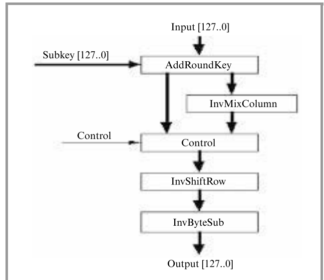
Fig. 11. The decryption round.
