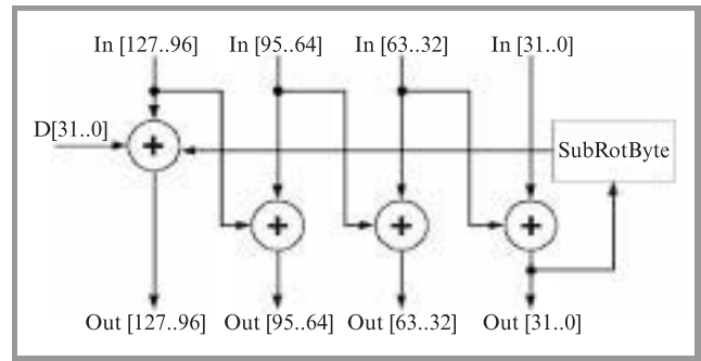
Fig. 15. The logical unit InvKeyRound.
