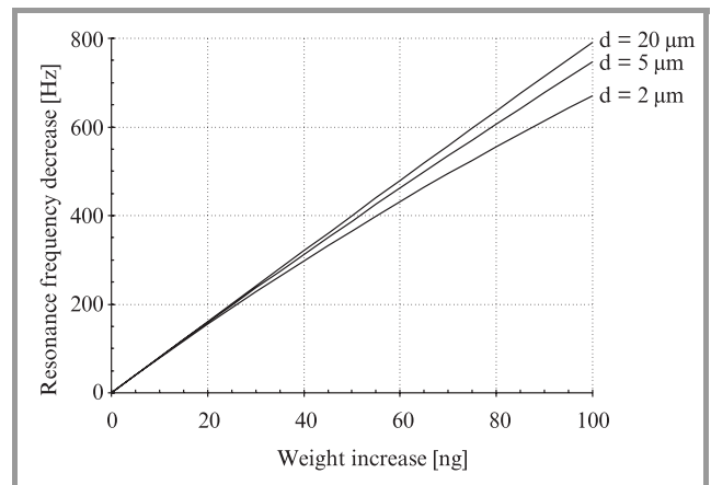
Fig. 3. Resonance frequency decreases due to adsorption for cantilevers (480 x 160 μm) and 2, 5 or 20 μm thick.
