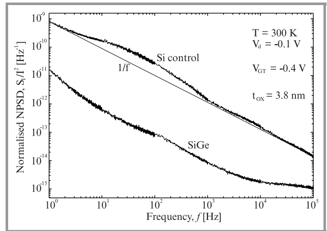
Fig. 15. Showing two orders of magnitude improvement in relative noise power spectral density (NPSD) in a Si/Si_{0.5}Ge_{0.5}/Si MOSFET as compared to a Si control (after Prest et al. [23]).
