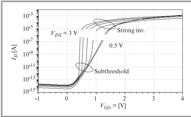
Fig. 1. A family of simulated I_D(V_{GFS}) characteristics of the PD SOI MOSFET ( W = 100 \mu\text{m} , L = 9.4 \mu\text{m} , T_{Ox_f} = 32.8 \text{ nm} , T_{Oxb} = 400 \text{ nm} , T_{Si} = 150 \text{ nm} , N_B = 9 \cdot 10^{16} \text{ cm}^{-3} , V_{GBS} = 0 \text{ V} ).
