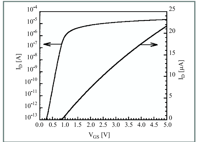
Fig. 3. Drain current as a function of gate voltage for BSIM3v3.2 modeled variable mobility long n -channel MOSFET, at V_{BS} = 0 , V_{DS} = 50 mV.
