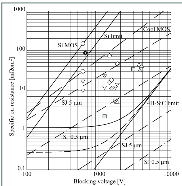
Fig. 11. Specific on-resistance of unipolar Si and SiC devices. The meaning of symbols is like in Fig. 8. The diamond with cross is a lateral MOSFET. The lines for SJ devices are shown for 5 \mu\text{m} and 0.5 \mu\text{m} wide regions (10 \mu\text{m} and 1 \mu\text{m} pitch, respectively).
