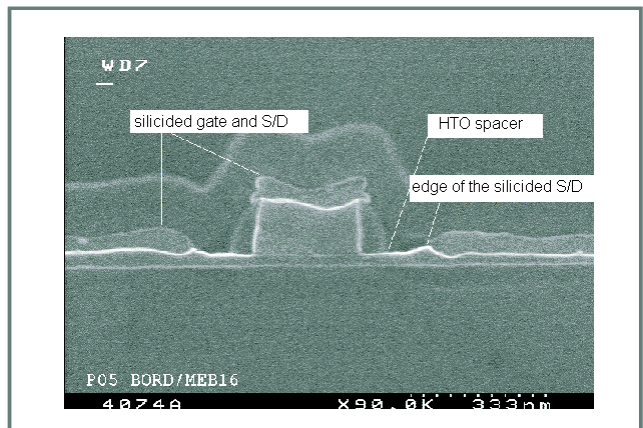
Fig. 5. Cross-section of a 0.25 \mu\text{m} FD SOI MOSFET (active silicon thin-film of 30 nm) with a recessed-channel process.
