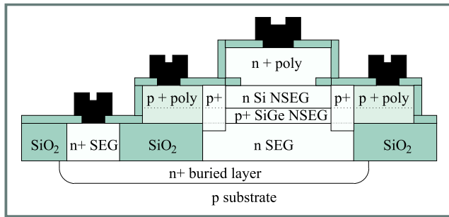
Fig. 4. Schematic diagram of SiGe HBT produced using selective epitaxy [17].
