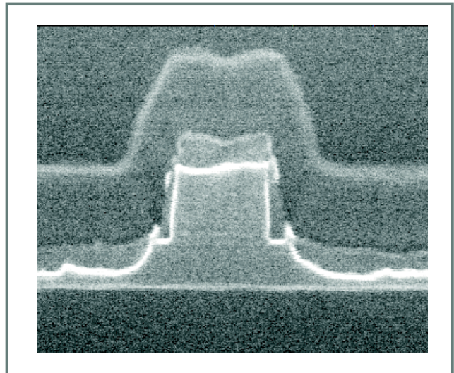
Fig. 4. Cross-section of a 0.25 \mu\text{m} PD SOI MOSFET (active silicon film of 100 nm) with a \text{TiSi}_2 silicidation process for the gate, drain and source areas.
