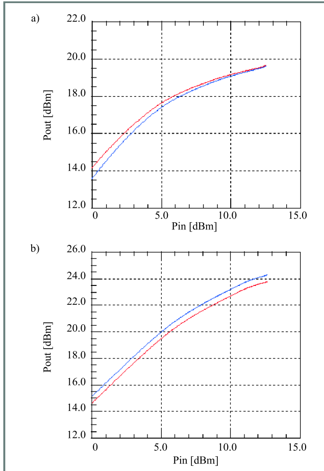
Fig. 11. Output power vs input power characteristics of the PA. Supply voltage is: (a) 1.5 V and (b) 2.7 V.
