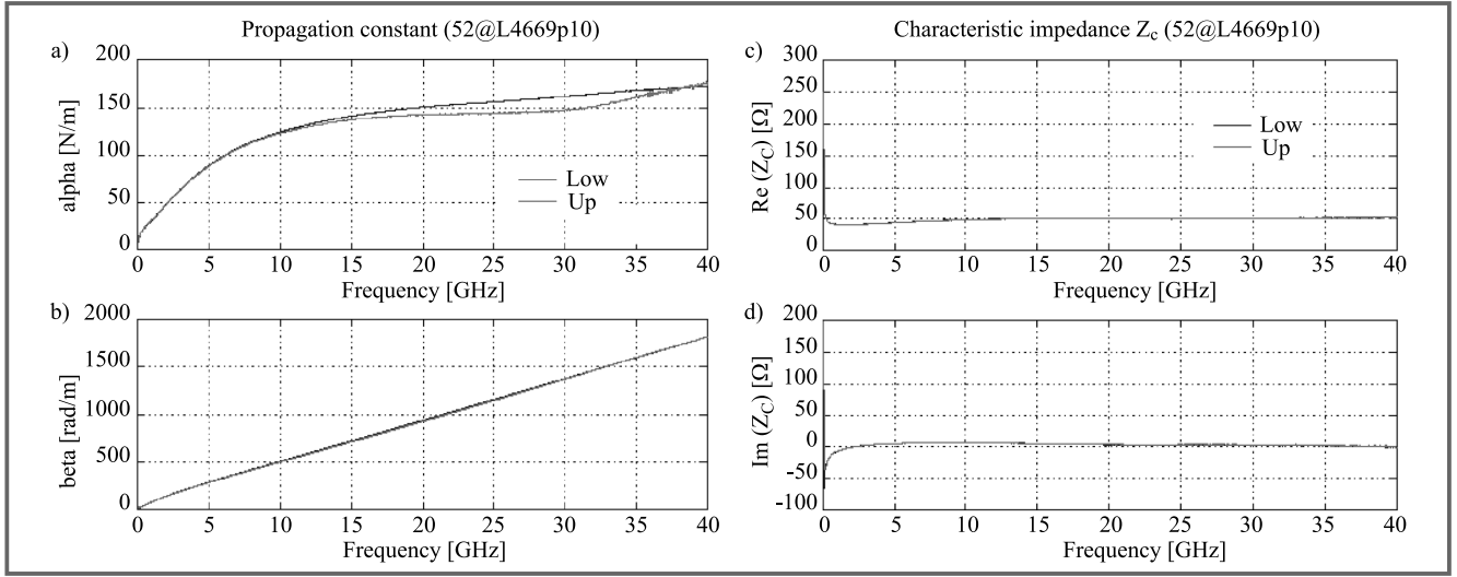
Fig. 4. Extracted complex propagation coefficient ( \gamma = \alpha + j\beta ) (a), (b) and complex characteristic impedance ( Z_c ) (c), (d) by considering the measured S-parameters of the short line (Up, called „through” in Fig. 2) and the long line (Low, called „line” in Fig. 2) in the calibration procedure.
