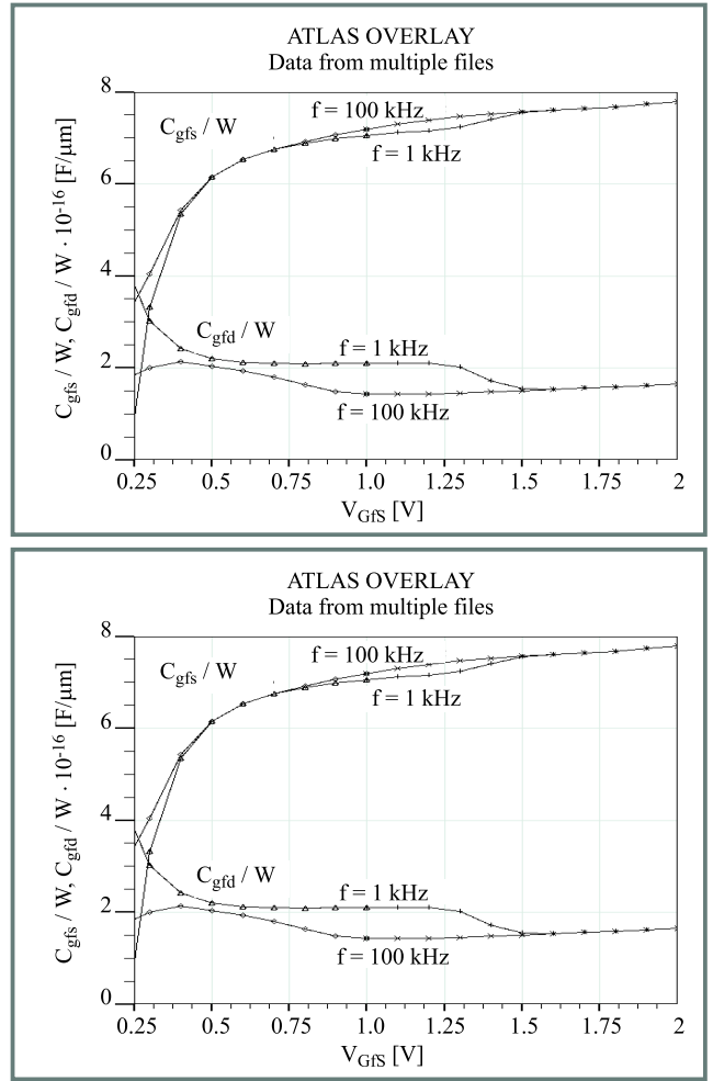
Fig. 8. C_{gfs}(V_{GFS}) determined numerically [8]. Device data: L = 0.6 \mu\text{m} , t_{Si} \approx 0.2 \mu\text{m} , t_{ox,b} \approx 0.4 \mu\text{m} , t_{ox,f} \approx 30 \text{ nm} , N_B \approx 5 \cdot 10^{16} \text{ cm}^{-3} .
