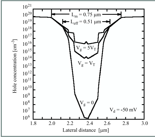
Fig. 15. Hole concentration at the interface of the p-channel MOSFET with L_m = 0.75 \mu\text{m} .
