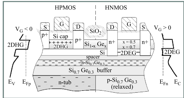
Fig. 10. Complementary HPMOSFET with a Si channel for the n-type and an SiGe channel for the p-type device. A common relaxed buffer is used for both transistors [34] (diagram reproduced from [32]).
