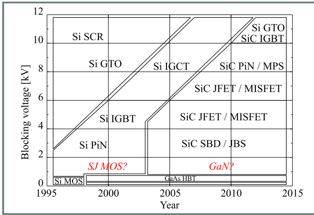
Fig. 10. Preferred device type and semiconductor material based on the data in Fig. 9.
