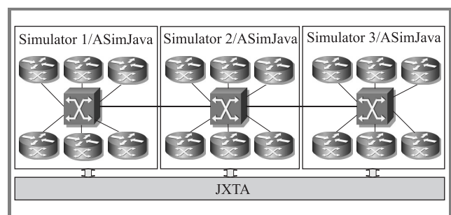
Fig. 5. Federated simulator of exemplified network E4.
