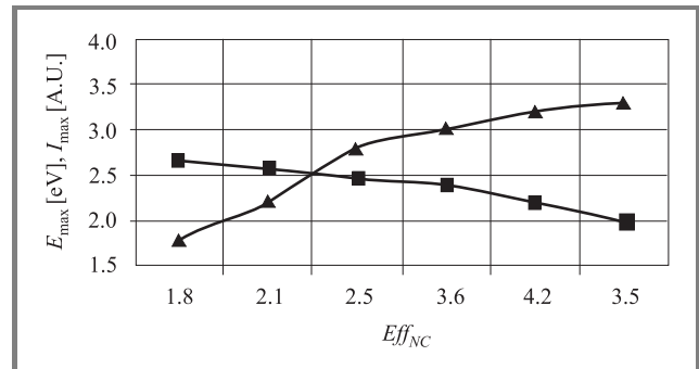
Fig. 2. Dependence of the low-energy photoluminescence spectral maxima (squares) and its relative intensities (triangles) on Eff_{NC} .
