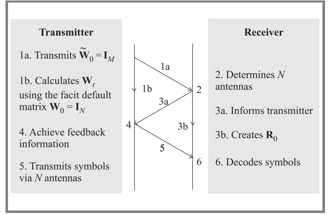
Fig. 2. The general (M, N; K) AST/DSTBC for the system using DSTBCs.
