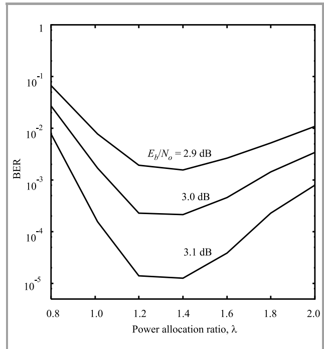
Fig. 14. Bit error rate performance versus the power allocation ratio when the code rate is 1/2 . The channel is assumed as the BSC.
