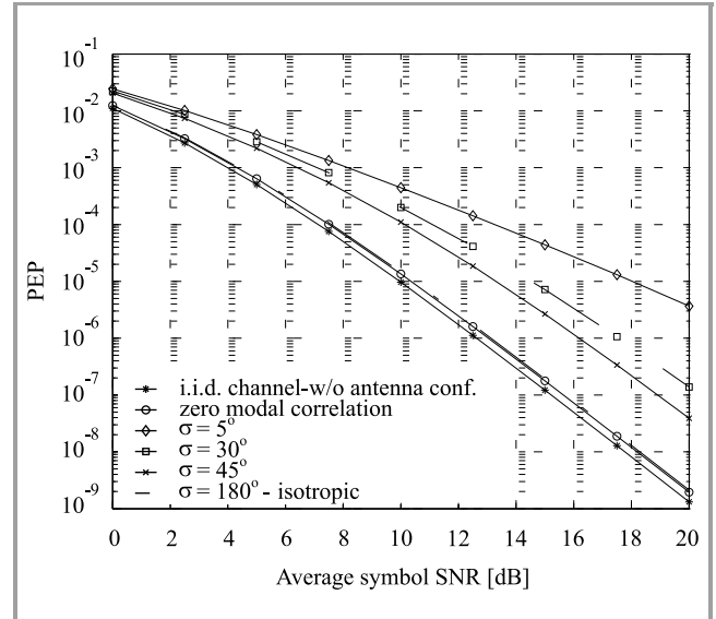
Fig. 5. Effect of receiver modal correlation on the exact-PEP of the 4-state QPSK space-time trellis code with 2-Tx antennas and 2-Rx antennas for the length 2 error event. Uniform limited power distribution with a mean angle of arrival \varphi_0 = 60^\circ from broadside and angular spreads \sigma = \{5^\circ, 30^\circ, 45^\circ, 180^\circ\} .
