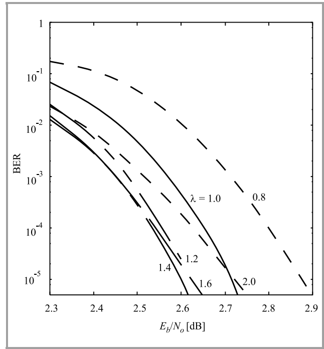
Fig. 13. Bit error rate performance versus E_b/N_0 for varying the power allocation ratio in the BSC. The code rate is set at 1/3 .
