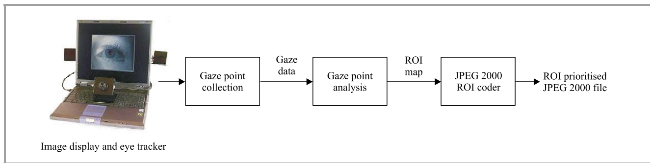
Fig. 1. Gaze-J2K system block diagram.
