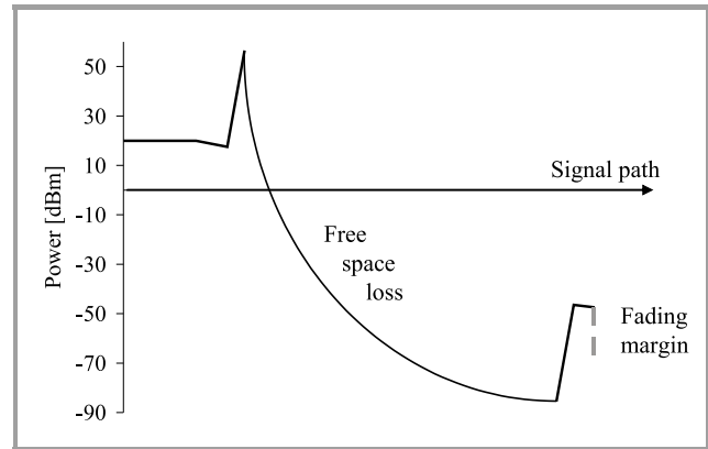
Fig. 3. Transmit/receive system and its link budget.
