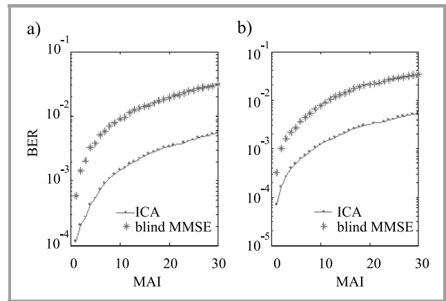
Fig. 7. Bit error rate versus MAI for \text{SNR} = 8 dB for various levels of signal power: (a) 15 dBw; (b) 5 dBw.
