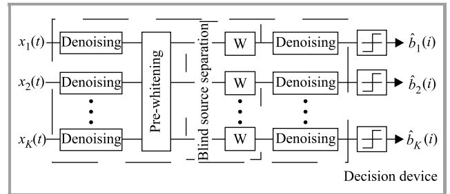
Fig. 3. The proposed blind receiver consists of PCA pre-whitening, ICA-BSS and wavelet denoising stages.
