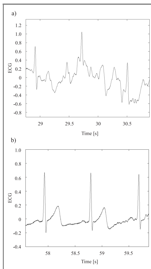
Fig. 5. ECG signal as recorded at rest with torsion artifacts: (a) without the membrane and (b) with the membrane. Signals have been recorded at Smartex in the IST European project WEALTHY framework.
