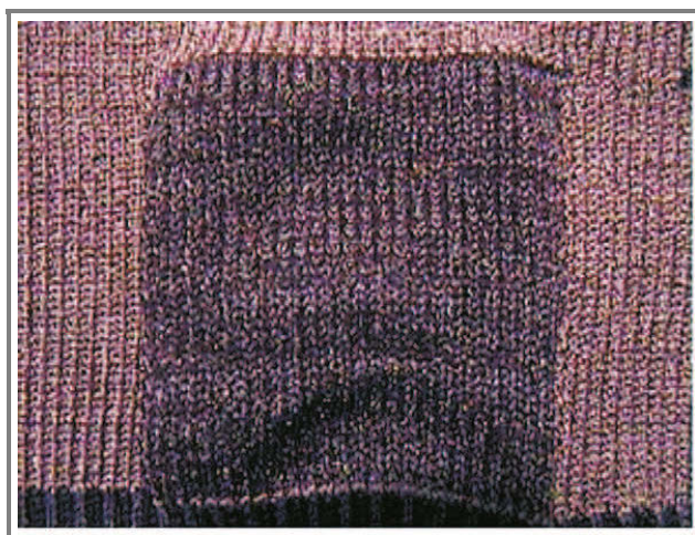
Fig. 4. ECG electrode woven in the fabric, as implemented in the IST European project WEALTHY.
