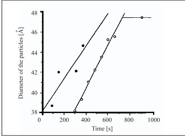
Fig. 4. A linear kinetic law is obtained for the growth of the nanoparticles The black circles stand for the 1:10 exchange ratio sample and the white circles for the 1:100 exchange ratio sample.
