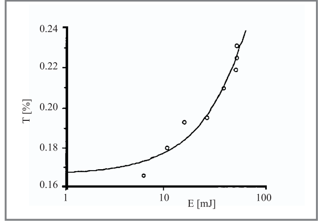
Fig. 7. Pulse energy dependent bleaching of the sample transmission T = \exp(-\alpha l) , and hence absorption saturation for a CdS Nafion membrane (exchange ratio of 1:10) with an emission peak at 700 nm
