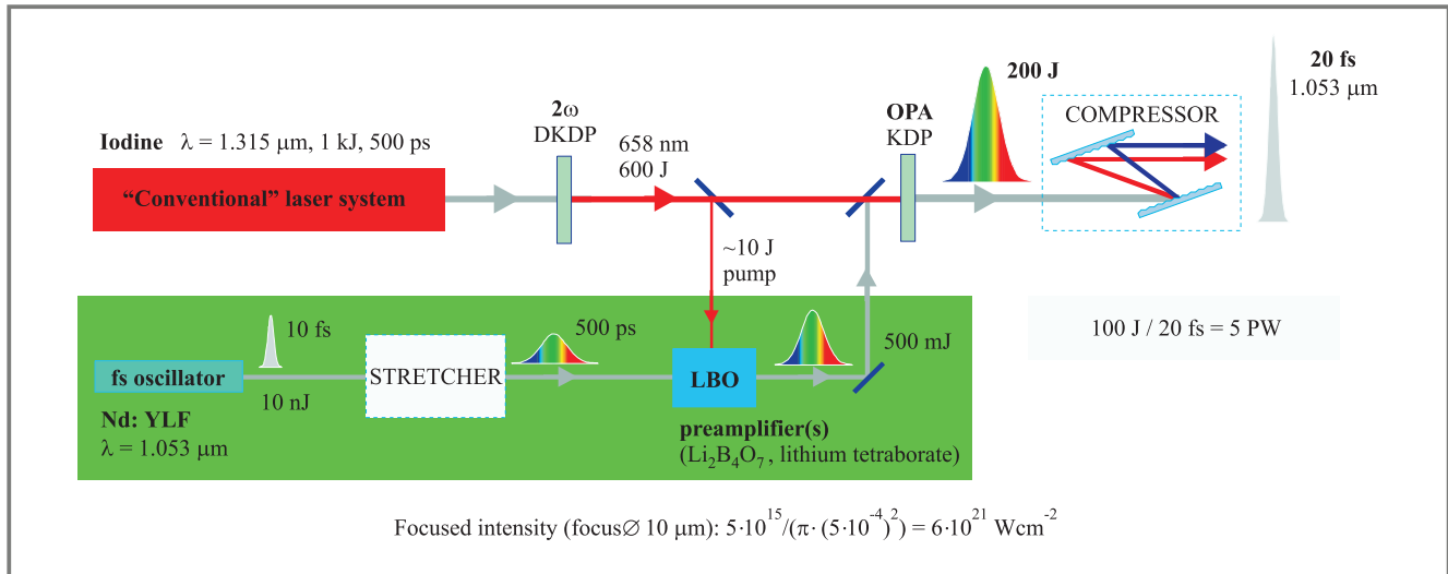
Fig. 12. Proposed scheme „Optical Parametric Chirped Pulse Amplification” of an iodine laser at PALS (Prague Asterix Laser System) (by courtesy of Bedrich Rus)
