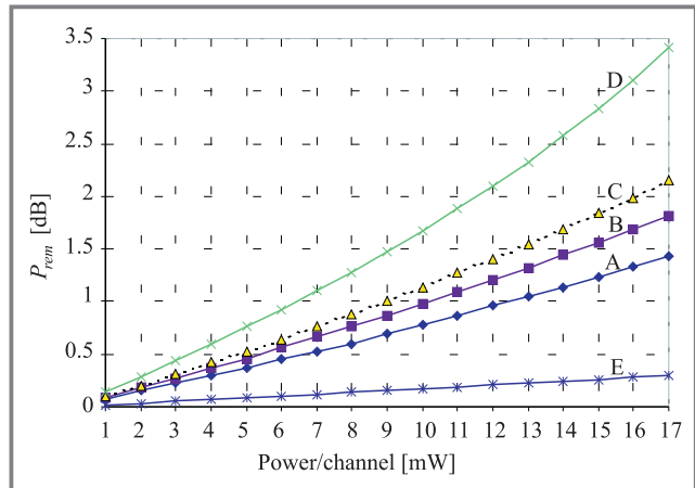
Fig. 1. Worst case power penalty introduced by SRS The fraction of the power P_{rem1} as a function of the power levels injected in each of the channels for various channel allocation schemes (A, B, C, D, E) calculated using formula (4).
