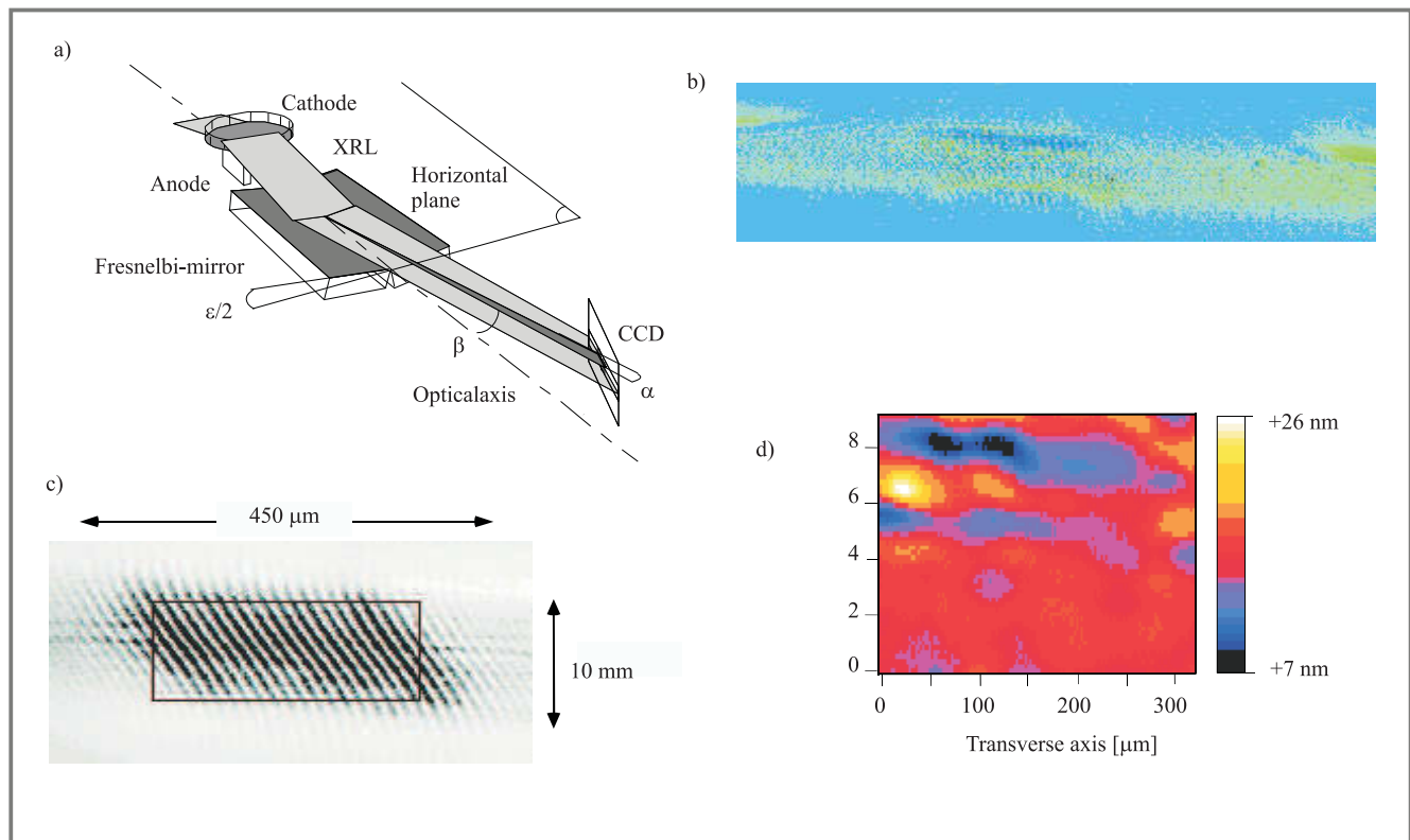
Fig. 13. Wavefront-division interferometric imaging of field-induced surface defects with X-ray lasers (by courtesy of F. Albert): a – eksperimental set up; b – interferogram subtraction between 14 MV/m and 0 MV/m (reference); c – example of experimental interferogram; d – height variation of the surface between 27 and 37 MV/m obtained by phase reconstruction.
