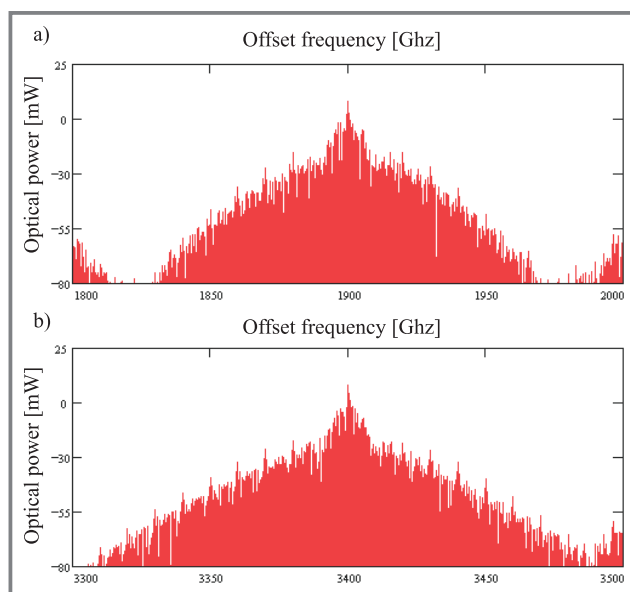
Fig. 5. The XPM optical spectrum degradation for two channels: with minimal (a) and maximal (b) distortion
