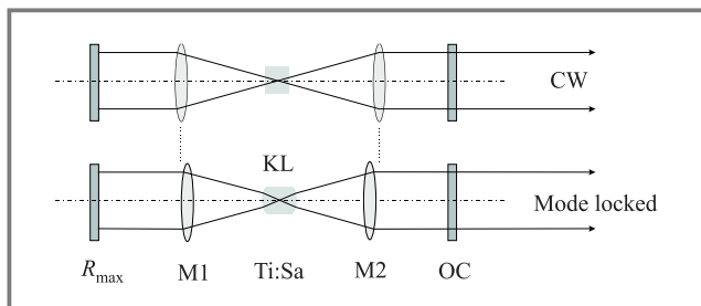
Fig. 2. Principle of the Kerr Lens Mode Locking
