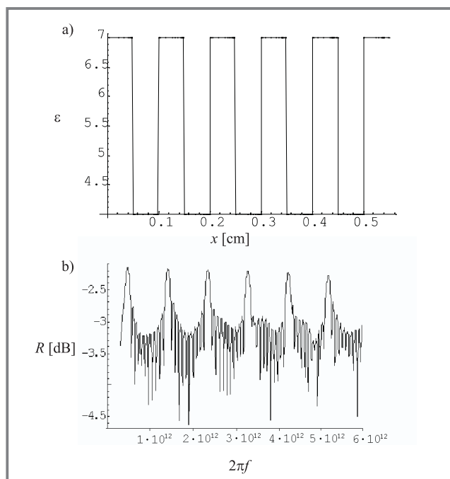
Fig. 3. Permittivity profile in the layer (a); reflection coefficient amplitude in dependence on the incident wave frequency (b)
