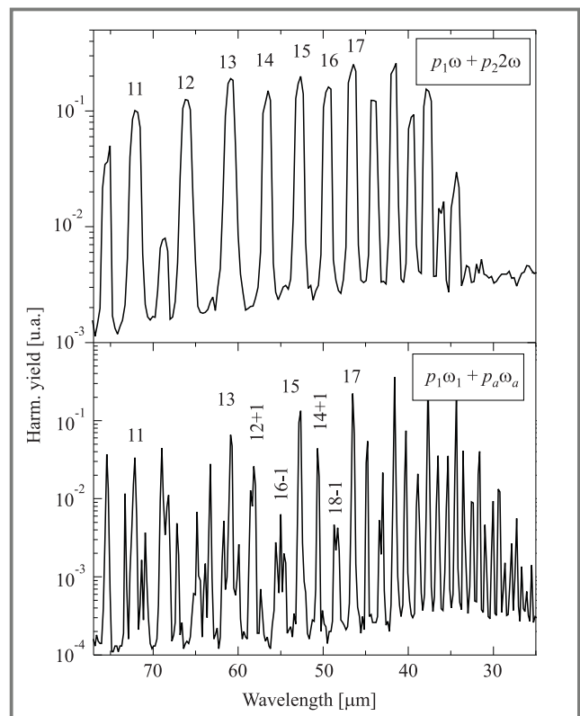
Fig. 9. High order harmonic spectra of the Ti:Sa laser obtained in Argon: top: fundamental and second harmonic of the pump laser are added to obtain even harmonics; bottom: the Ti:Sa fundamental is added to an OPA to obtain fine tunability (by courtesy of B. Carré and F. Salieres)
