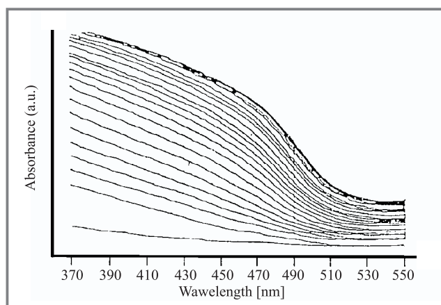
Fig. 3. Evolution of the absorption spectrum with time of exposure of a 1:100 exchange ratio Cd membrane exposed to dried hydrogen sulphide
