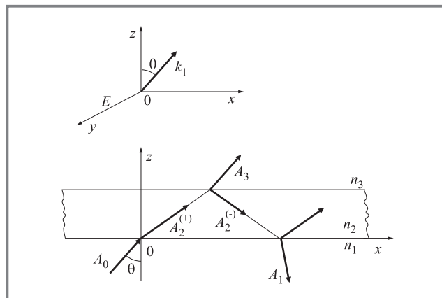
Fig. 1. Schematic diagram of the thin-film amplifier-oscillator
