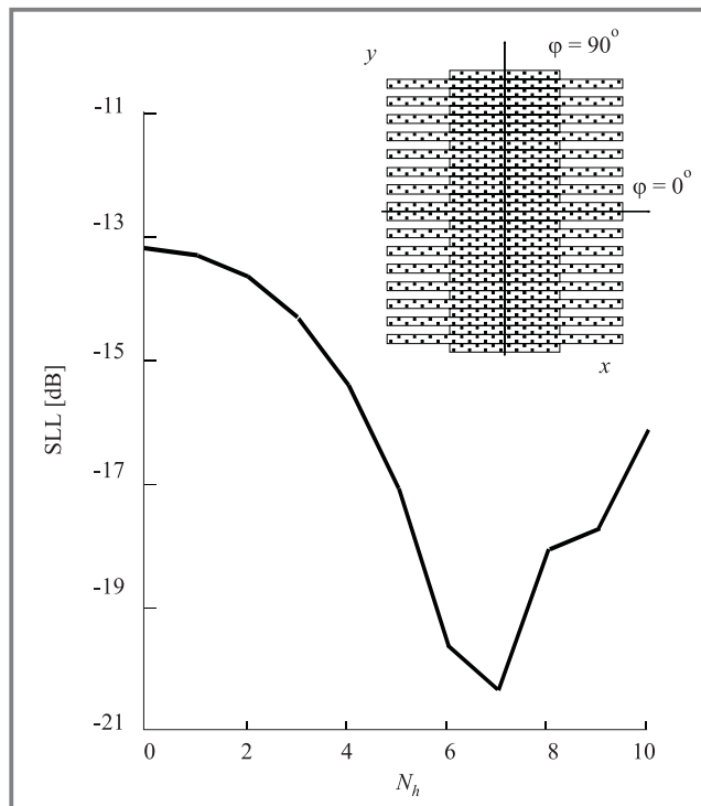
Fig. 1. SLL distribution in rectangular array with comb
