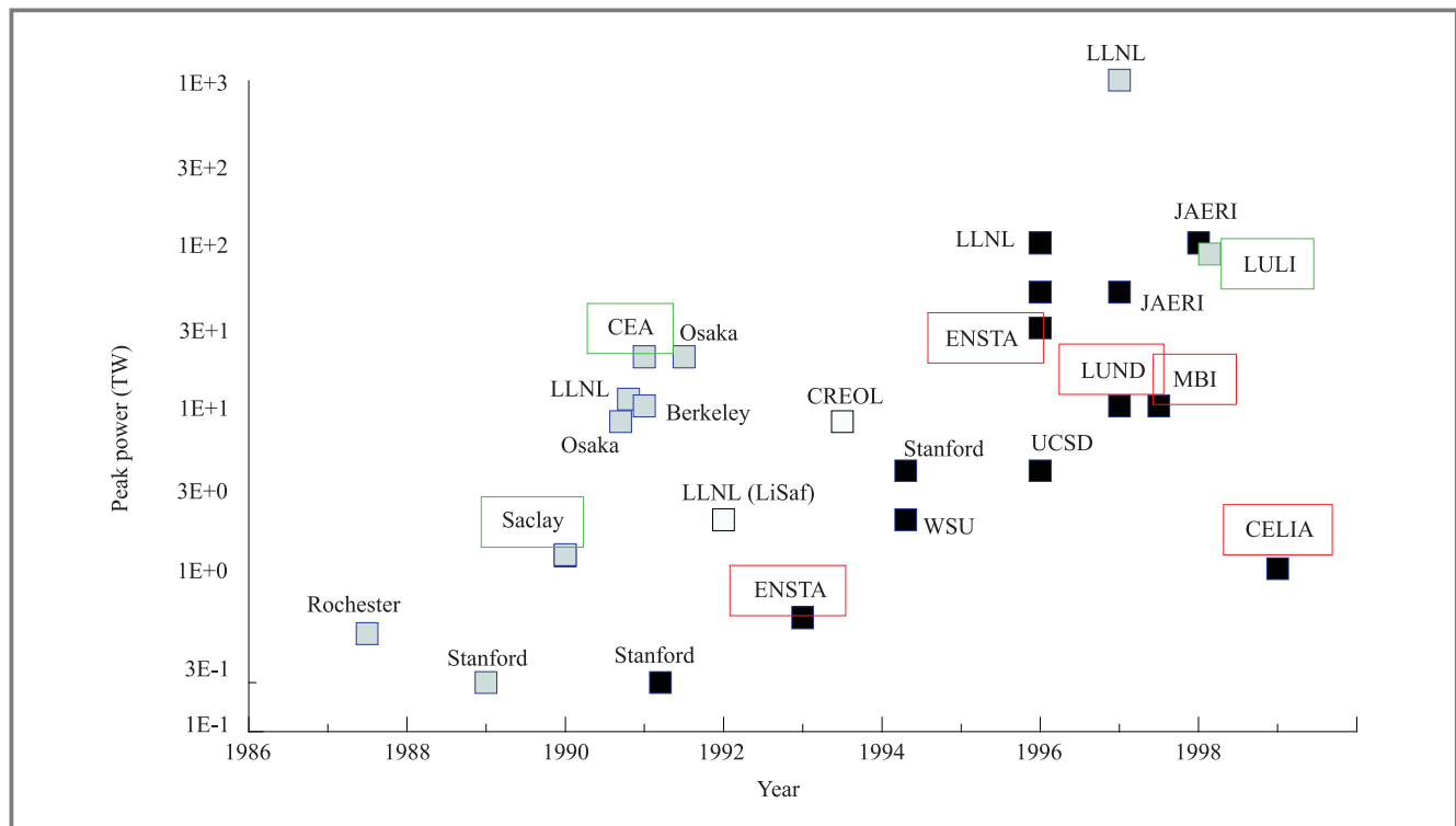
Fig. 5. Past evolution of the peak power of high intensity CPA based laser systems (by courtesy of C. Leblanc and C. Barty) In grey: Nd:Glass, Empty: LiSaf, Black: Ti:Sa; European based systems are circled.
