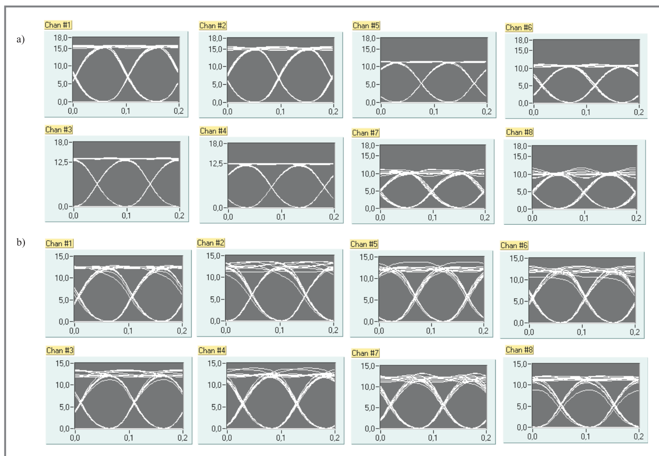
Fig. 2. The eye diagrams of the detected signal for equidistant channel spacing (a) and non-equidistant channel spacing (b)
