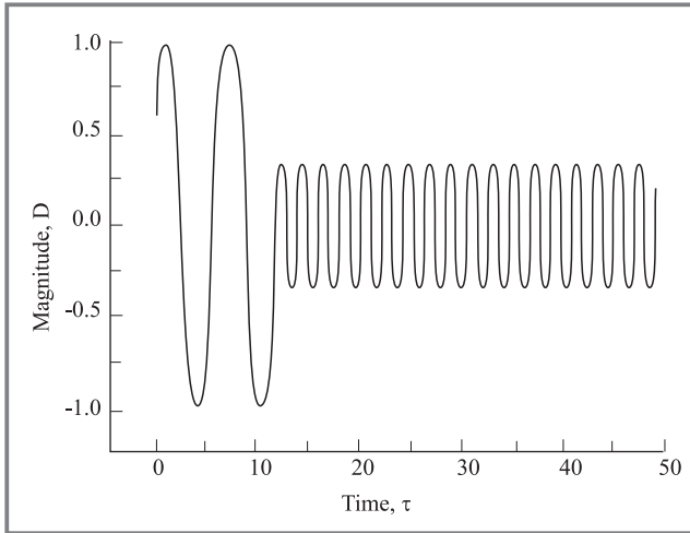
Fig. 1. The frequency shift with time jump of permittivity at \tau_0 = 12 when \varepsilon_1/\varepsilon = 9
