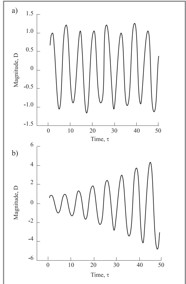
Fig. 3. The field transformation for great modulation depth of the permittivity: (a) g = \sqrt{2} , b = 0.9 , (b) g = 1.9 , b = 0.7
