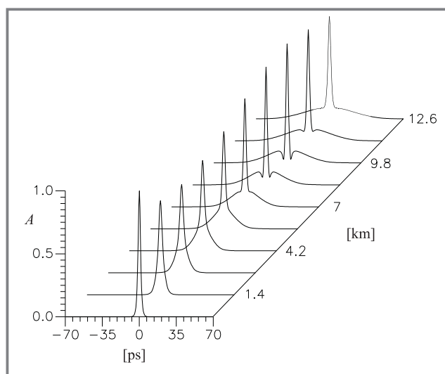
Fig. 1. Evolution of the fundamental soliton when C = 0.5
