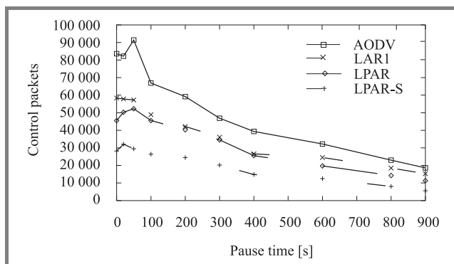
Fig. 10. CTRL packets for 300 N and 10 s.
