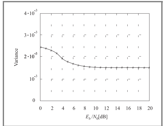
Fig. 8. Variance as a function of E_b/N_0 for M_I = 512 and N = 128 .
