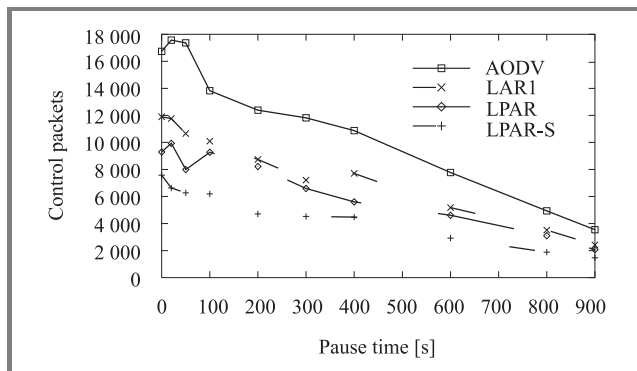
Fig. 9. CTRL packets for 50 N and 10 s.
