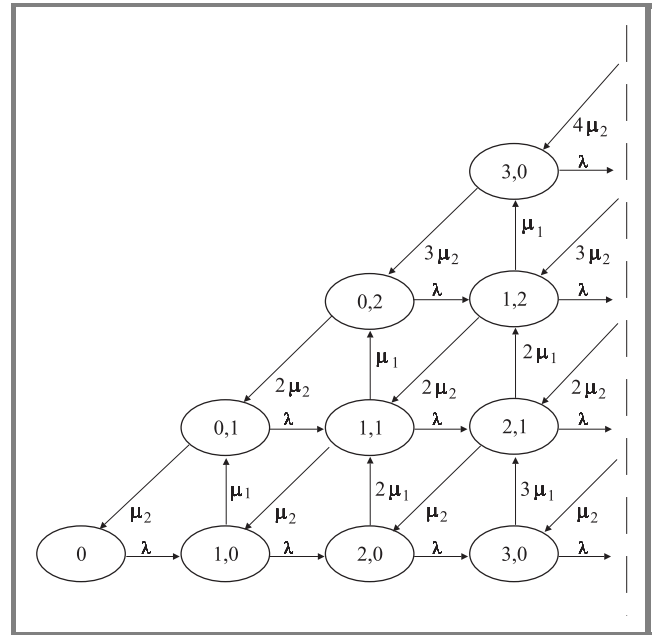
Fig. 2. First few states of the M/PH/n/n QBD process.
