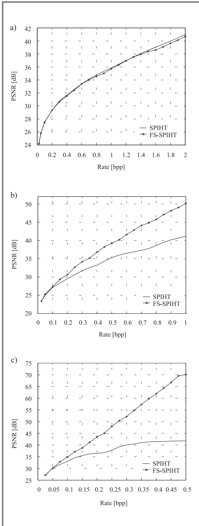
Fig. 5. Comparison of rate-distortion results for the Goldhill test image at different spatial resolution levels: (a) level 1 (original image size 512 \times 512 ); (b) level 2 ( 256 \times 256 ); (c) level 3 ( 128 \times 128 ).
