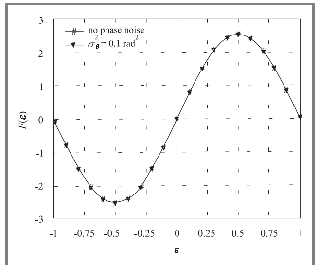
Fig. 5. Average SPI as a function of frequency offset in presence of phase noise for N = 128, 300 symbols.
