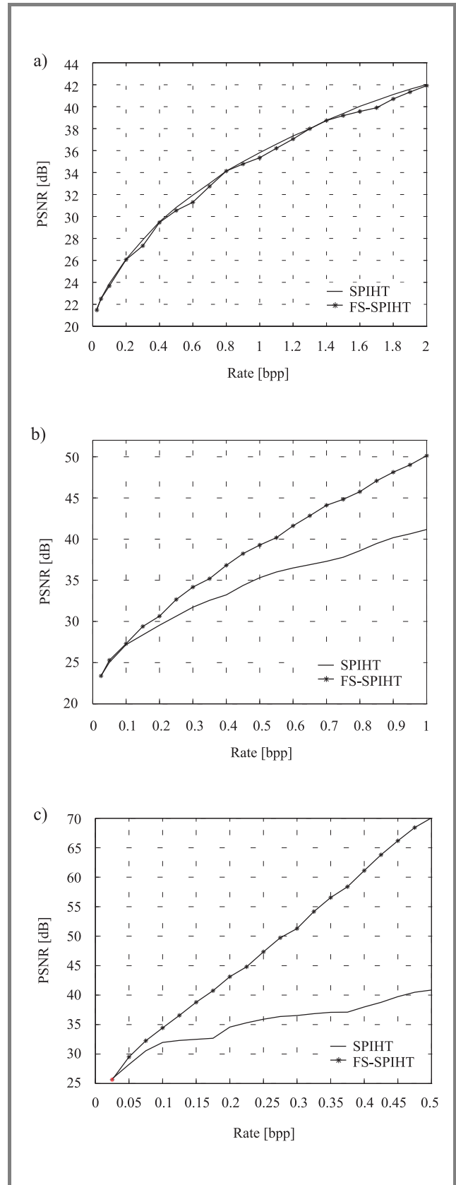
Fig. 6. Comparison of rate-distortion results for the Barbara test image at different spatial resolution levels: (a) level 1 (original image size 512 \times 512 ); (b) level 2 ( 256 \times 256 ); (c) level 3 ( 128 \times 128 ).
