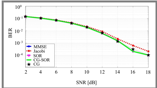
Fig. 7. BER versus SNR plots of JA, SOR, CG, and the proposed CG-SOR algorithm for an N \times U 128 \times 16 mMIMO system configuration and k = 4 , under 64-QAM.
