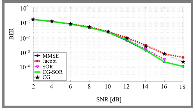
Fig. 6. BER versus SNR plots of JA, SOR, CG, and the proposed CG-SOR algorithm for an N \times U 128 \times 16 mMIMO system configuration and k = 3 , under 64-QAM.
