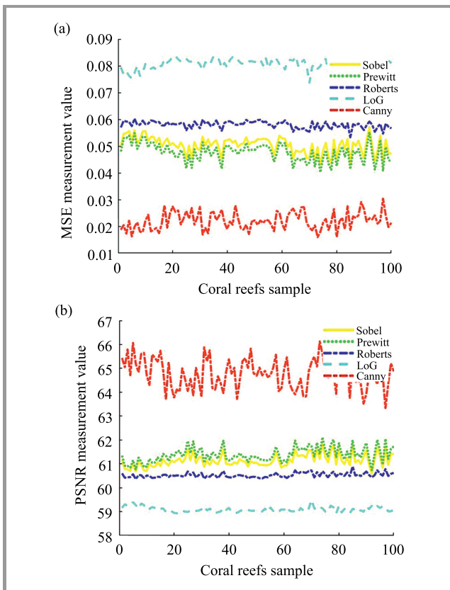
Fig. 8. (a) MSE and (b) PSNR analysis of various edge detection algorithms with median filtering by adding Gaussian noise.
