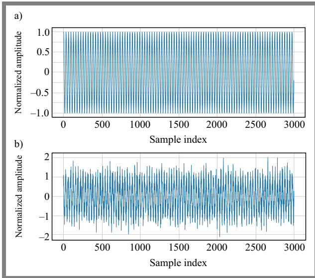
Fig. 9. Legitimate user RF signal a) and PUE attack RF signal b).
