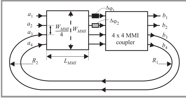
Fig. 1. The structure of a microring resonator based on 4 × 4 MMI couplers.
